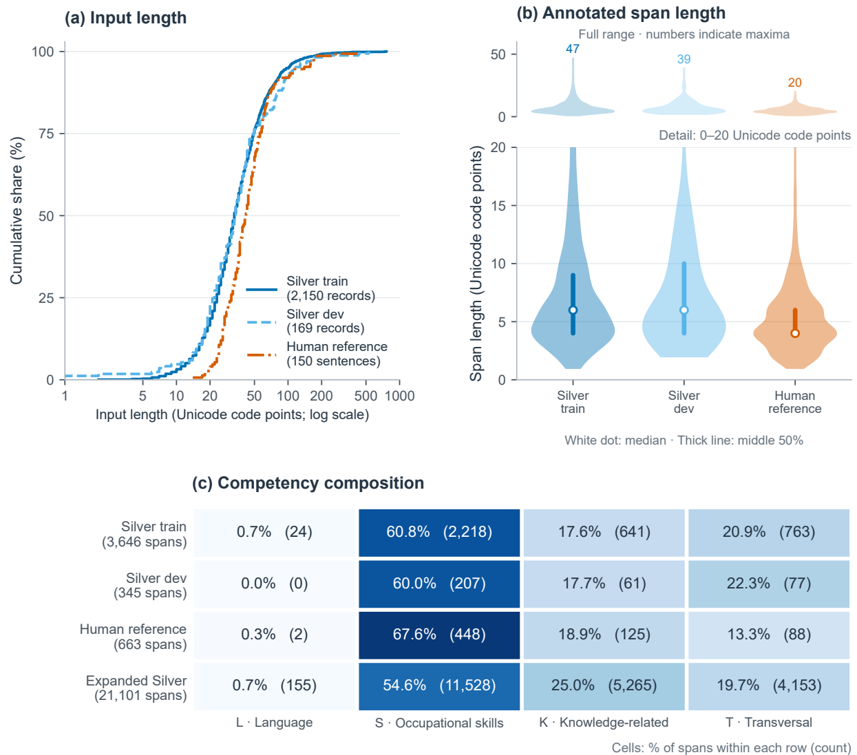
Figure 4. Dataset characteristics: (a) input lengths; (b) annotated span lengths; and (c) competency-type distributions, including the full adopted expanded pool. Silver train/dev denote the Qwen and encoder splits. Lengths are measured in Unicode code points, including punctuation and spaces. All records contribute, including those with identical text.
