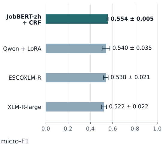
Figure 5. Typed exact-span micro-F1 on the same 150-sentence human reference set. Panel (a) shows single prompted runs; panel (b) shows means with sample standard deviations over seeds 42, 43, and 44. Training and inference settings differ across model families. Detailed scores appear in Tables 17, 18, and 8.
