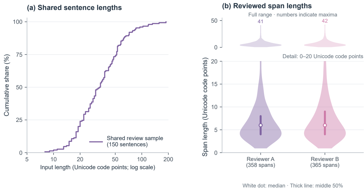
Figure 8. Length distributions in the additional assisted-review sample. Panel (a) uses the same 150 sentences for both reviewers; panel (b) shows their separate annotation layers, with 358 spans for A and 365 for B. Densities use all observed spans with equal maximum widths. The overview shows the full range of span lengths, while the detail view focuses on 0–20 Unicode code points. Dots mark medians, and thick lines mark the middle 50%. Supervision and human-reference distributions appear in Figure 4; reviewer-specific type counts appear in Table 13.
