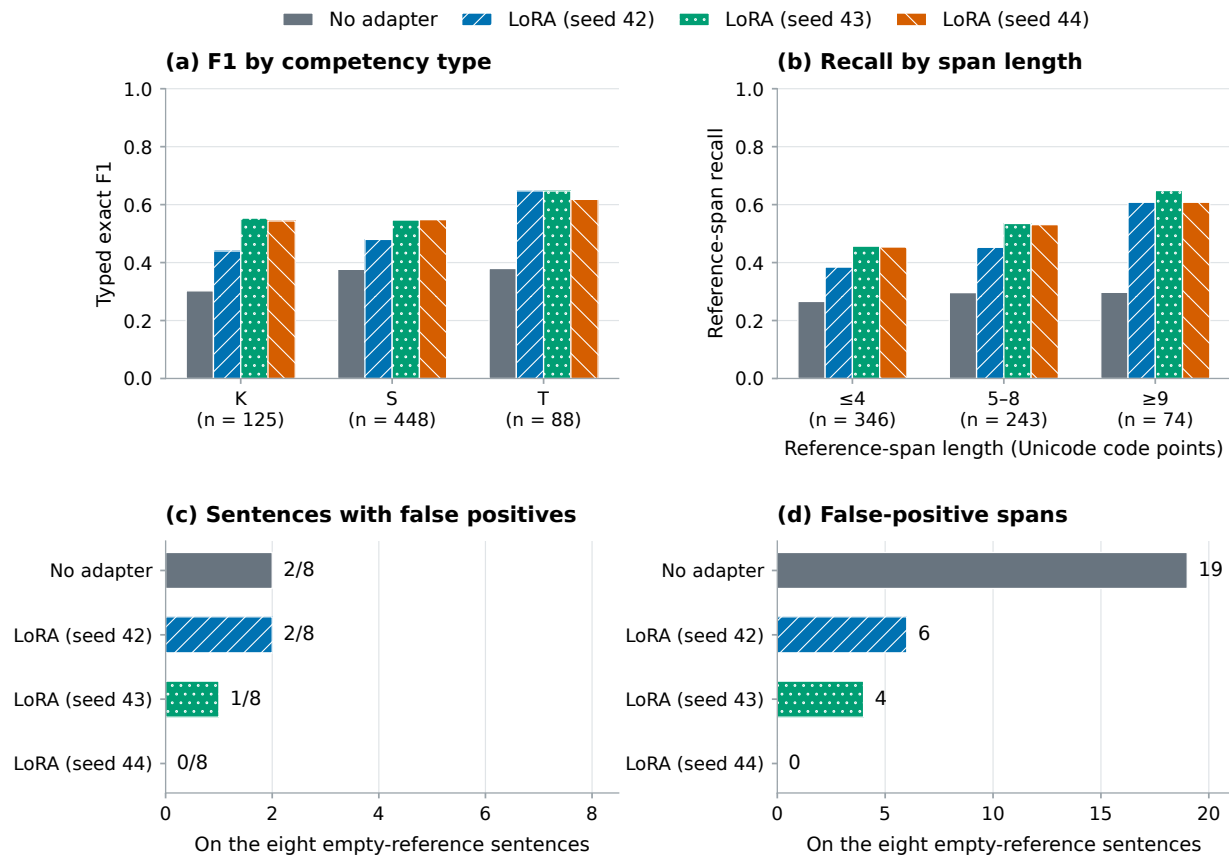
Figure 6. Qwen diagnostics on the human reference set: (a) typed exact-span F1 for K/S/T; (b) recall by reference-span length ( n : reference spans); (c–d) false positives on eight sentences with no reference spans, counted by sentence and span.
