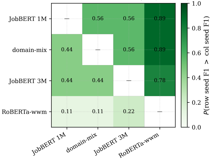
Gold v2 encoder seed win-rate (n=3; not ASO)
