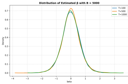
Figure 1.1 Distribution of estimated \beta with different sample size T
