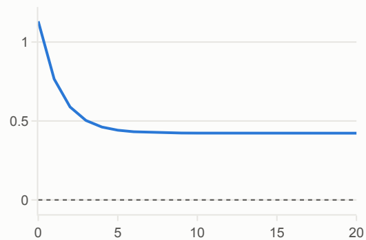
Shock to GDP growth first in the recursive order
