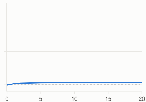
Shock to energy demand growth second in the recursive order
