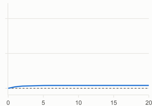
Shock to the interest rate fifth in the recursive order
