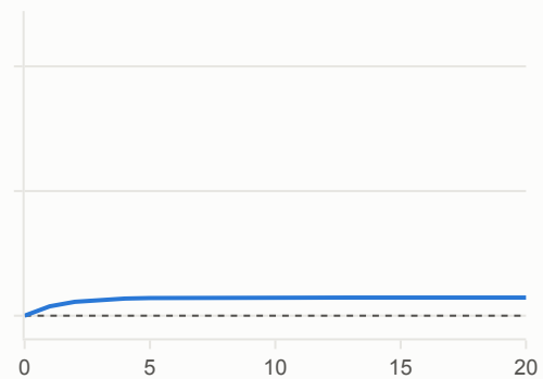
Shock to employment change third in the recursive order
