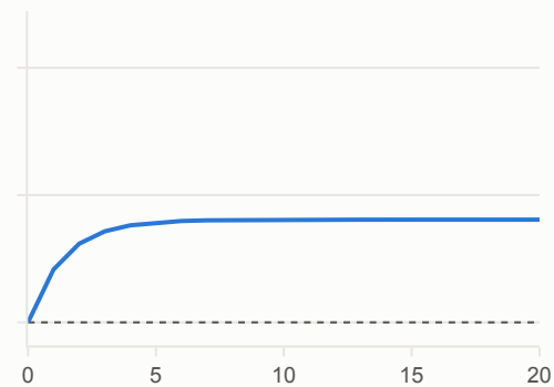
Shock to inflation fourth in the recursive order
