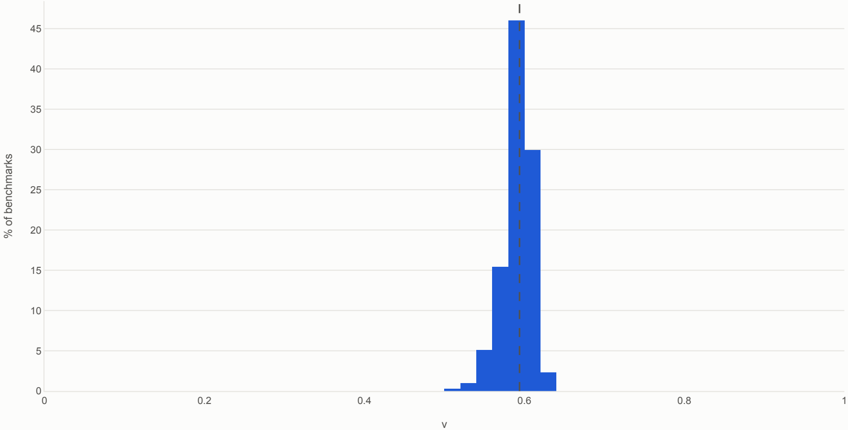
Local projection, both states: v over the runs of cop_0191, 1,000 benchmarks. Dashed line: median, 0.594
