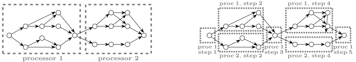
FIGURE 2.1. Example partitioning (left) and a scheduling (right) of the same computation, with 2 processors. While the partitioning is completely balanced (it assigns 9 vertices to both parts), it does not allow any parallelism: all the vertices of processor 1 need to be finished before any vertex of processor 2 can begin executing. In contrast to this, scheduling also assigns the vertices to (super)steps. In (super)steps 2 and 4, the two processors can indeed execute the assigned workloads in a parallel manner.
