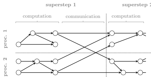
FIGURE 1.1. Here's an example DAG-BSP-schedule picture, if needed. Old descriptions in comments.
