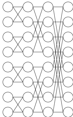
(A) Directed acyclic graph representation of a fast Fourier transform on an input of length eight. Connections should be read from left to right.
