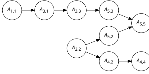
FIGURE 7.1. Dependencies in the forward-substitution algorithm, Algorithm 7.1, of the matrix A in Equation 7.2.
