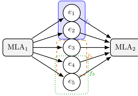
FIGURE 7.4. Simplified hypergraph of two MoE layers. Each colored group has its own frequency f_e . The ILP uses these frequencies to decide which experts and MLAs should be placed on the same device.
