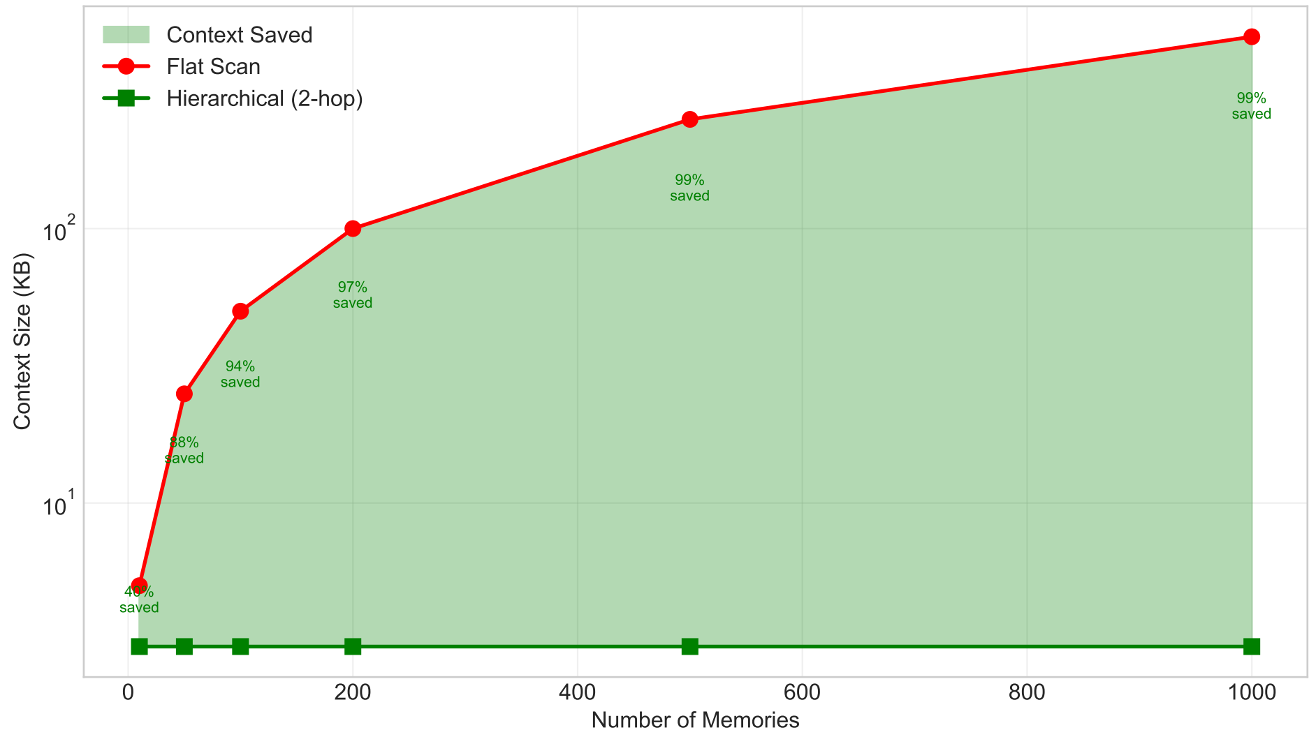
Retrieval Context Size: Flat vs Hierarchical Index
