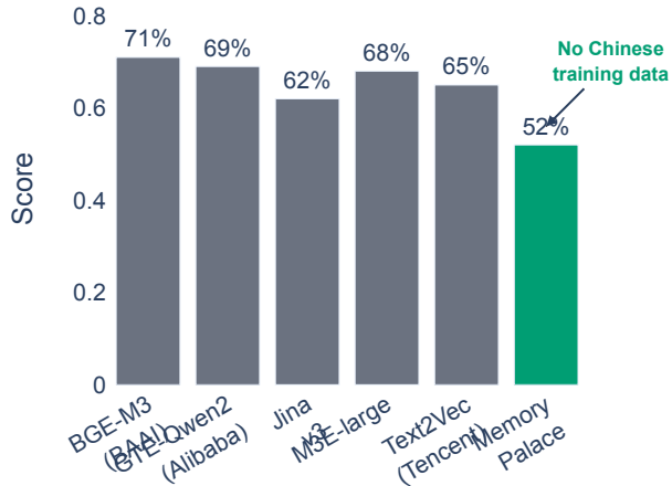
C-MTEB (Chinese-specific)
