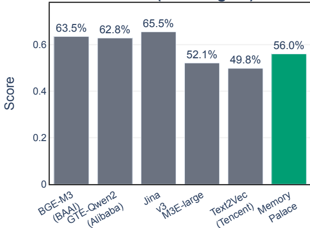
MTEB (Multilingual)
