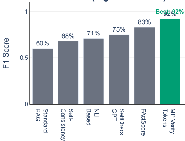
F1 Score (higher is better)
