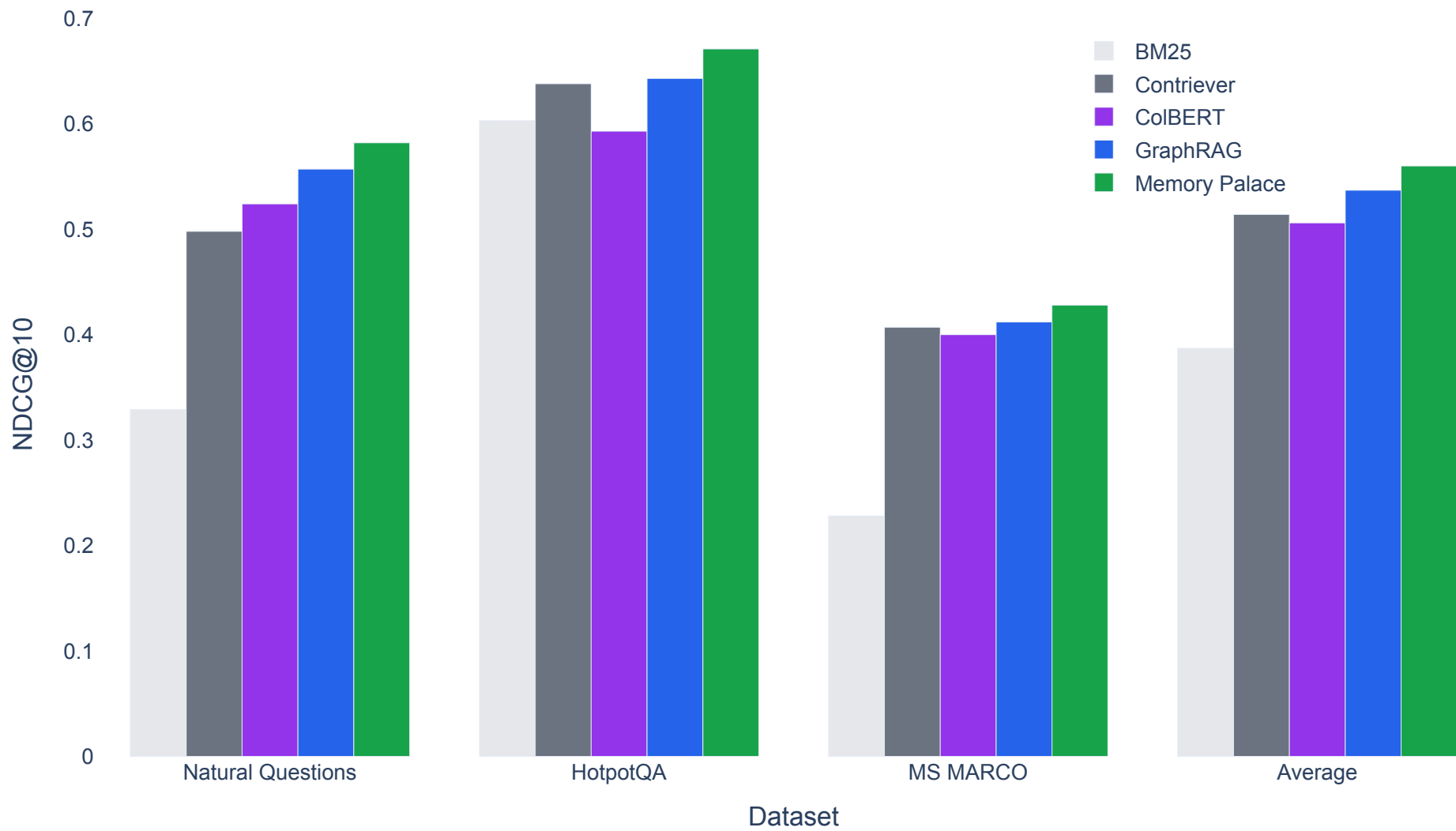
BEIR Benchmark: NDCG@10 by Dataset
