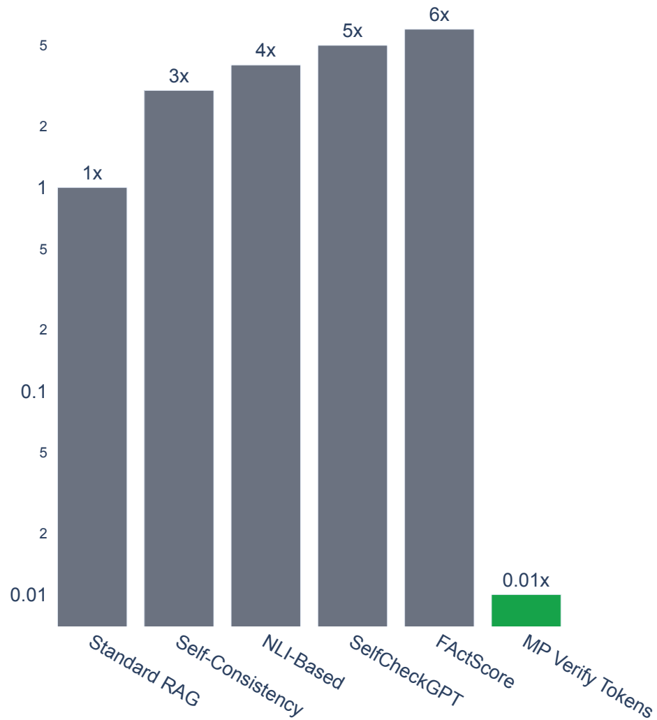
Compute Cost (relative)
