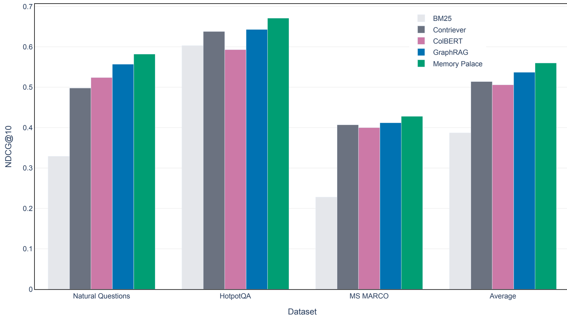
BEIR Benchmark: NDCG@10 by Dataset
