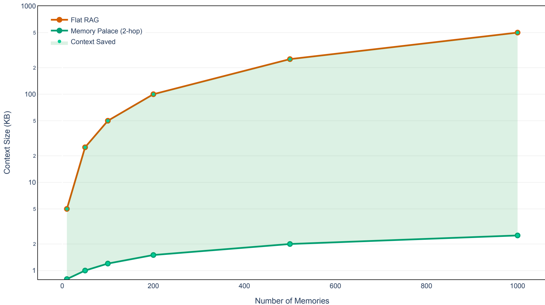
Context Size Scaling: Flat vs Hierarchical Retrieval
