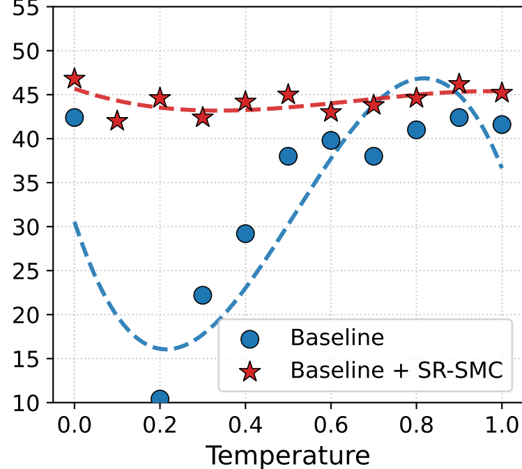
Dream-7B (MATH)
