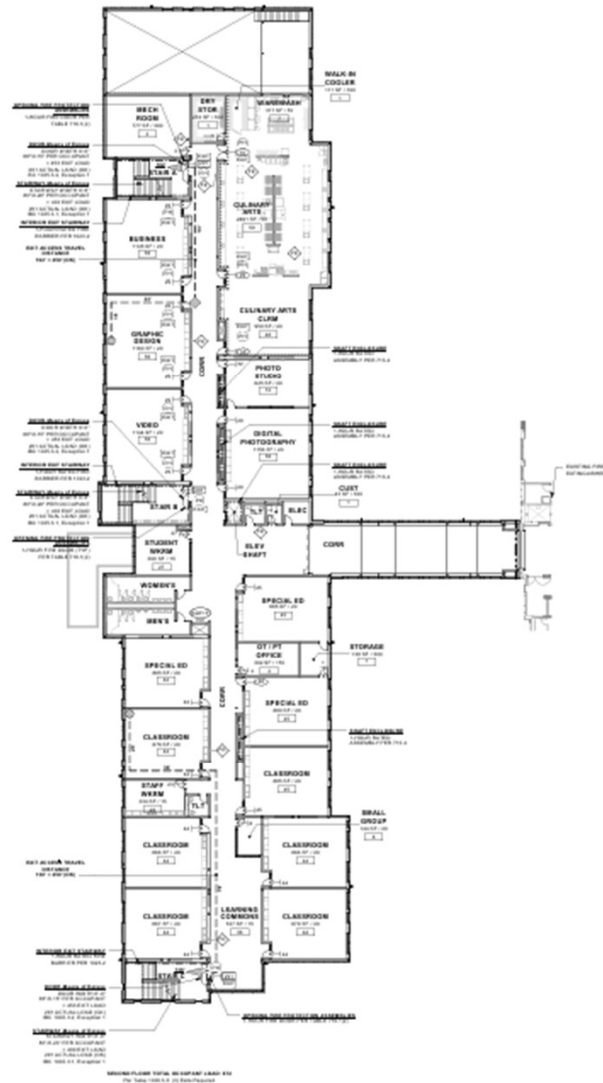
SECOND FLOOR EGRESS PLAN SCALE: 1/8" = 1'-0"
