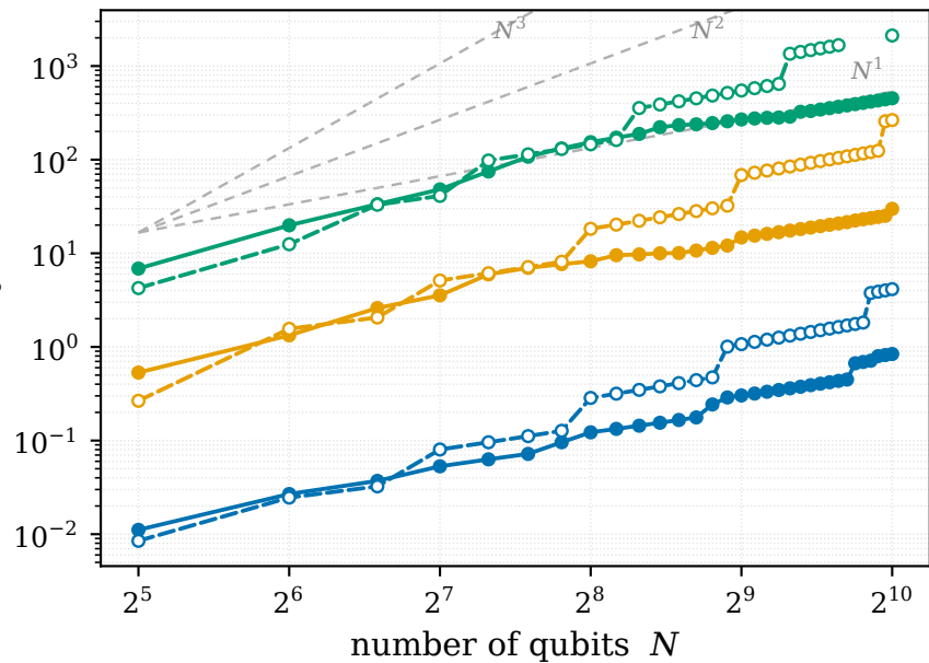
memory (MB)
