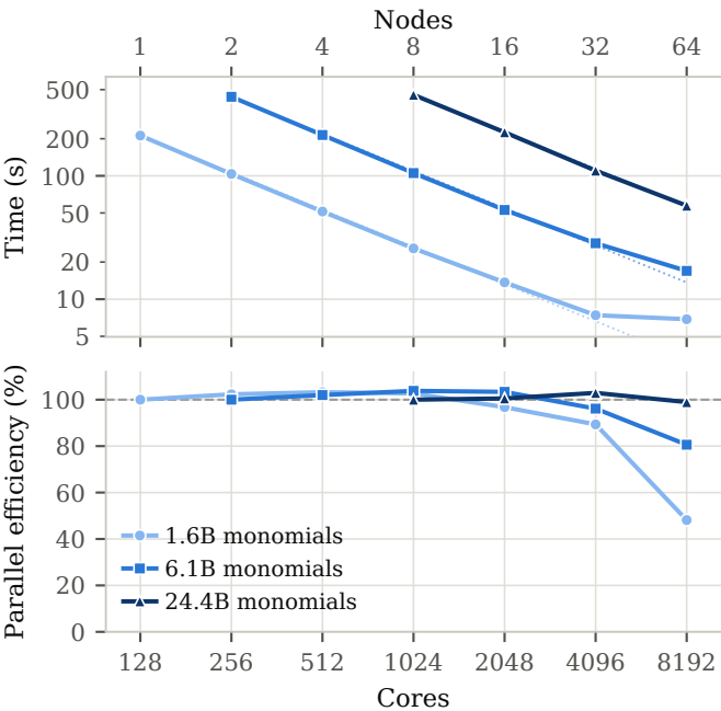
Strong scaling
