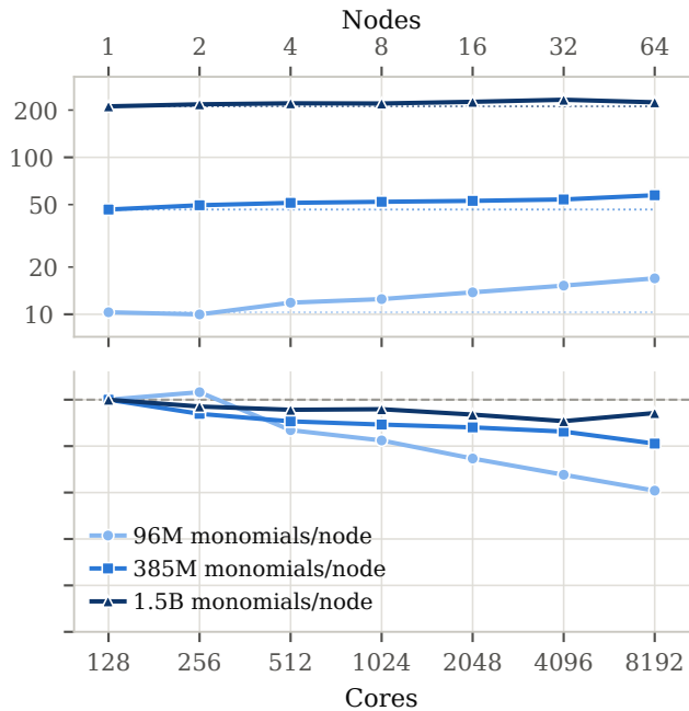
Weak scaling
