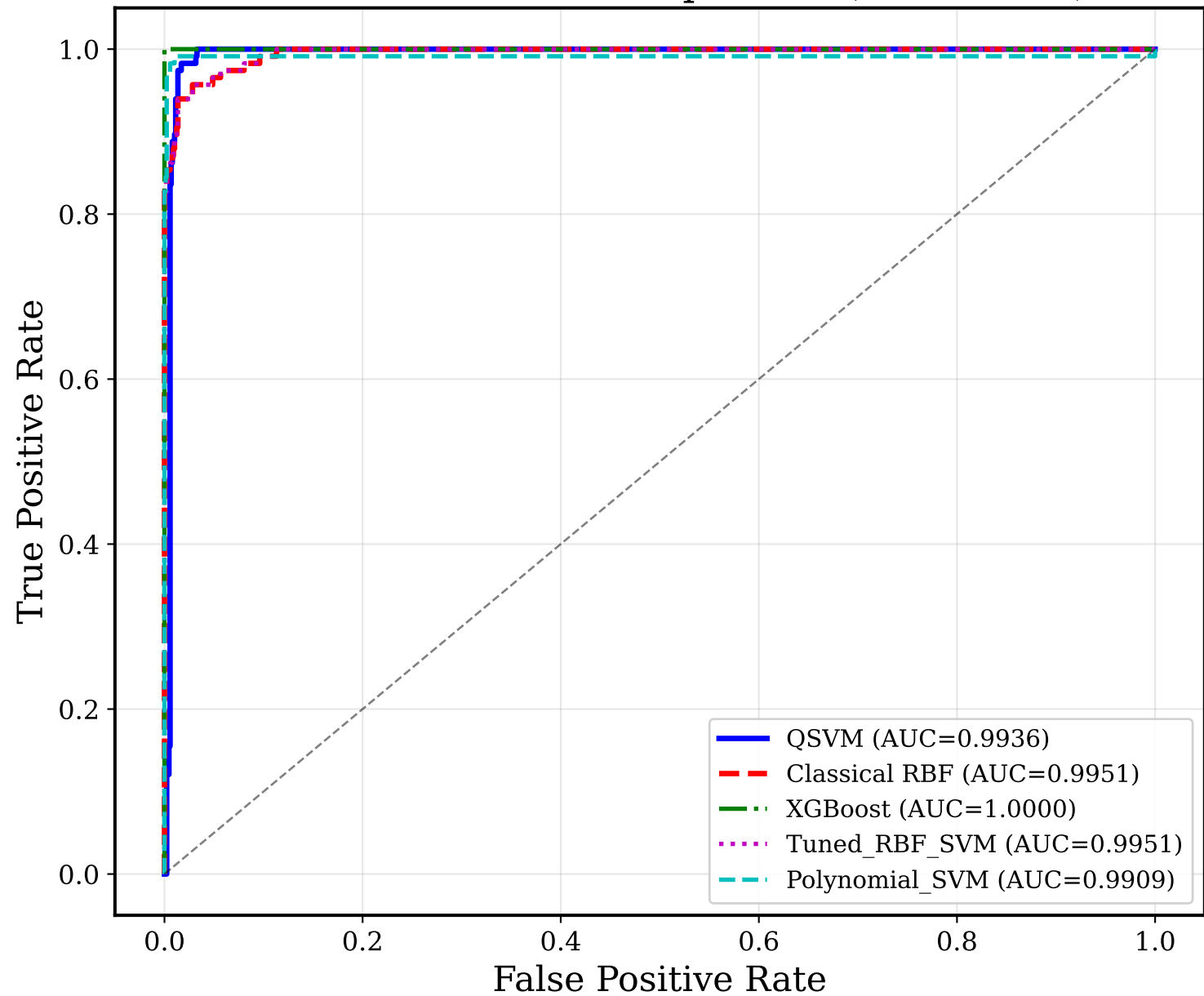
SWaT ROC Curve Comparison (Simulation)
