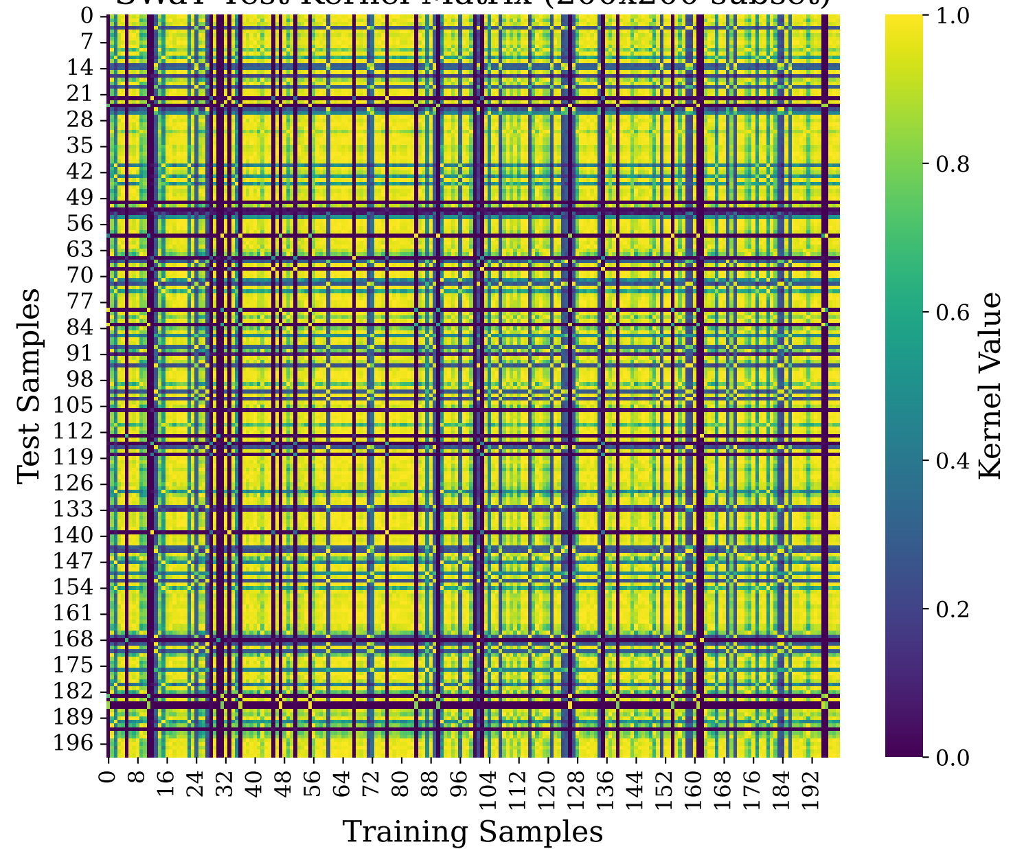
SWaT Test Kernel Matrix (200x200 subset)
