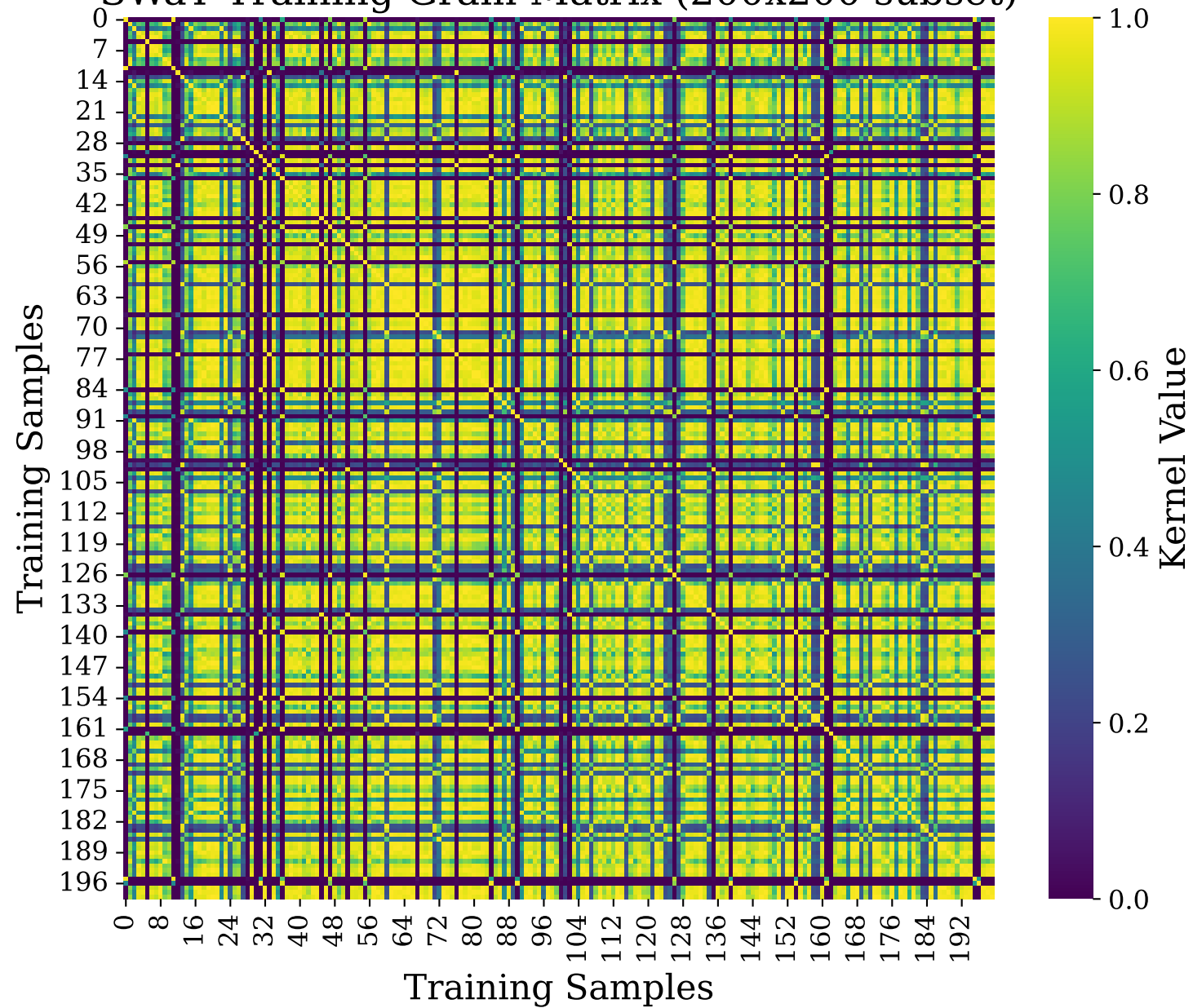
SWaT Training Gram Matrix (200x200 subset)
