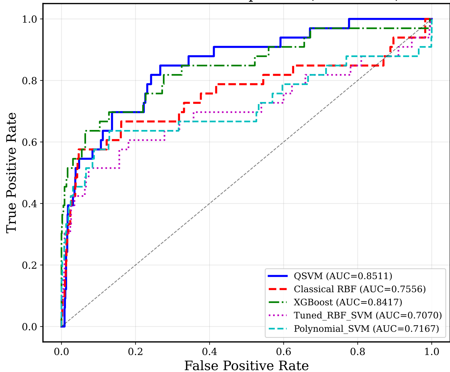
HAI ROC Curve Comparison (Simulation)
