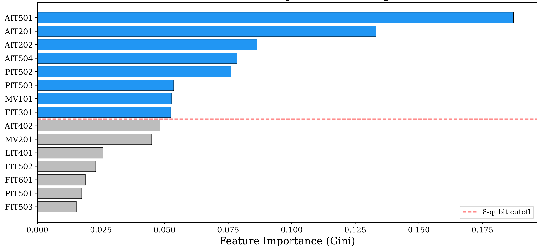
SWaT Feature Importance Ranking
