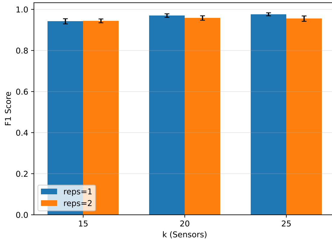
Ablation 2: Feature Map Repetitions
