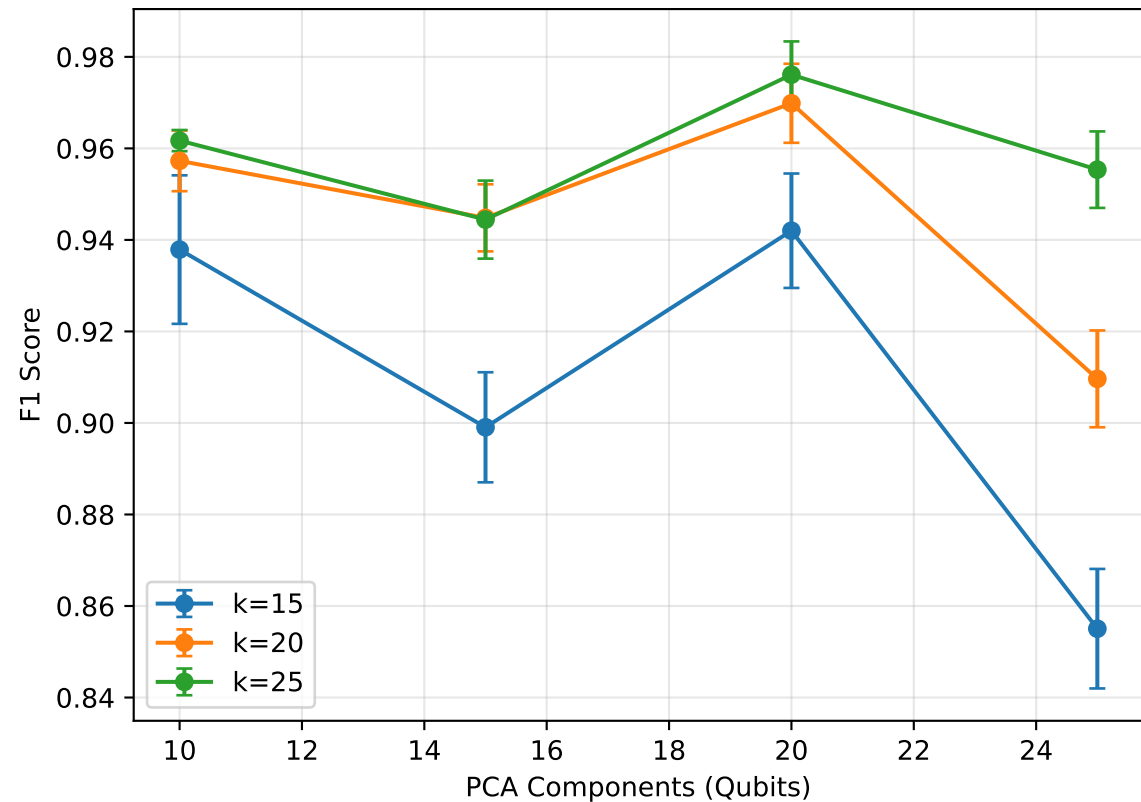
Ablation 1: PCA Components
