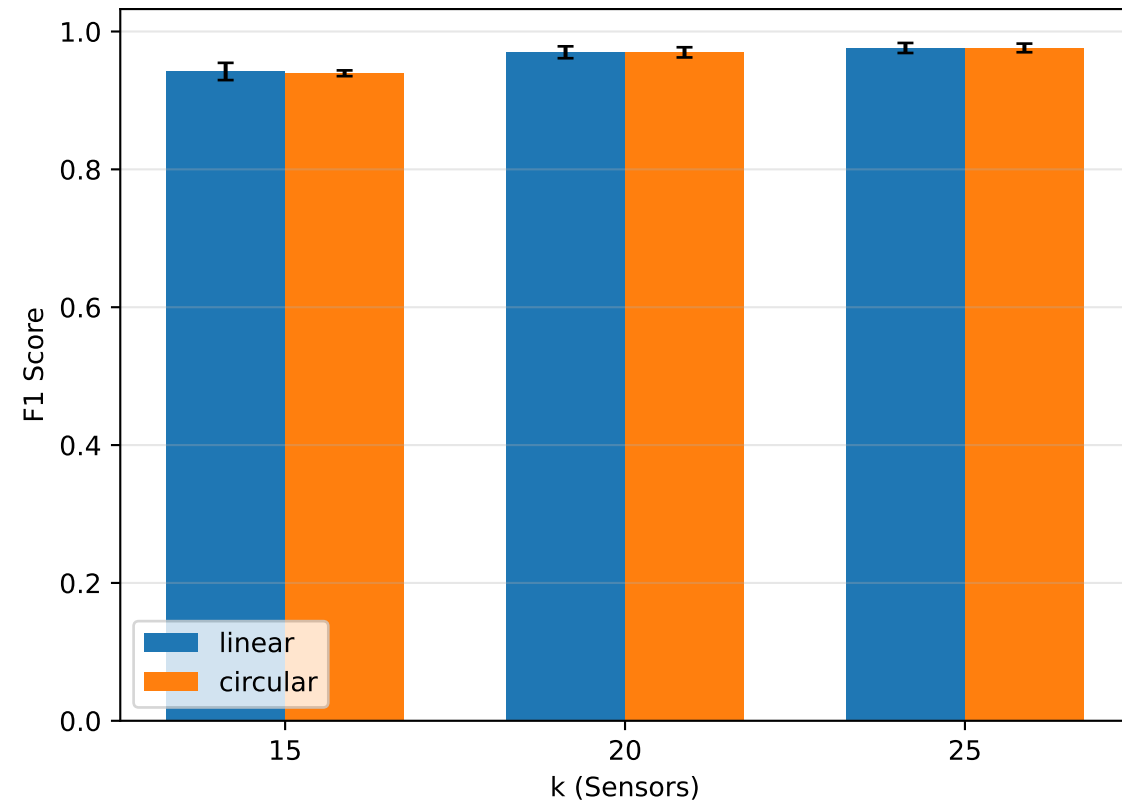
Ablation 3: Entanglement Type
