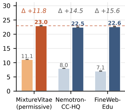
Reasoning, 4K, after Tulu3 SFT
