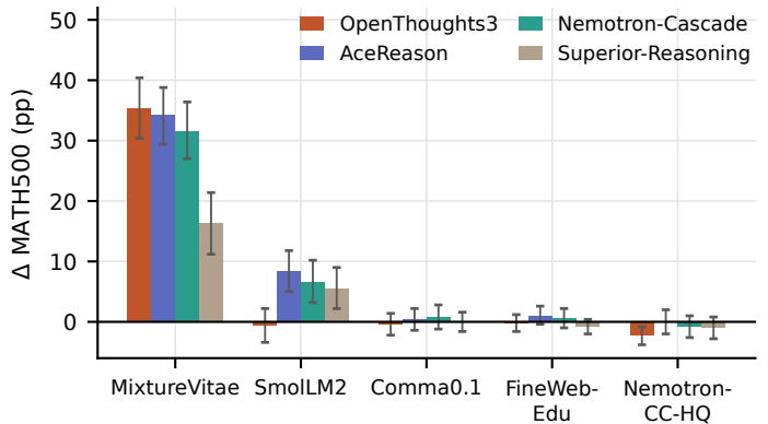
Four reasoning corpora, from the Tulu3 SFT checkpoint
