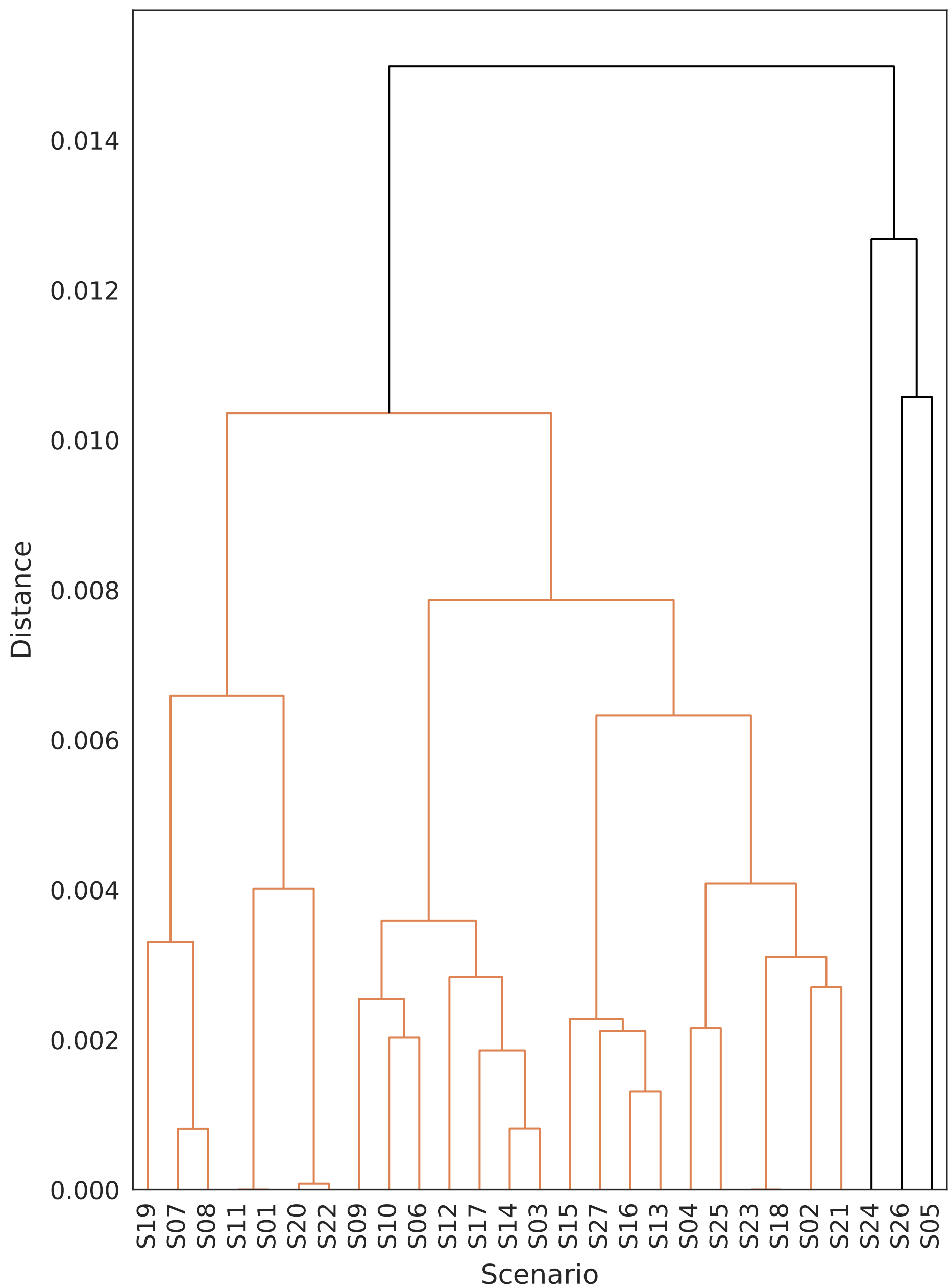
GHGAbateFMs Hierarchical Dendrogram
