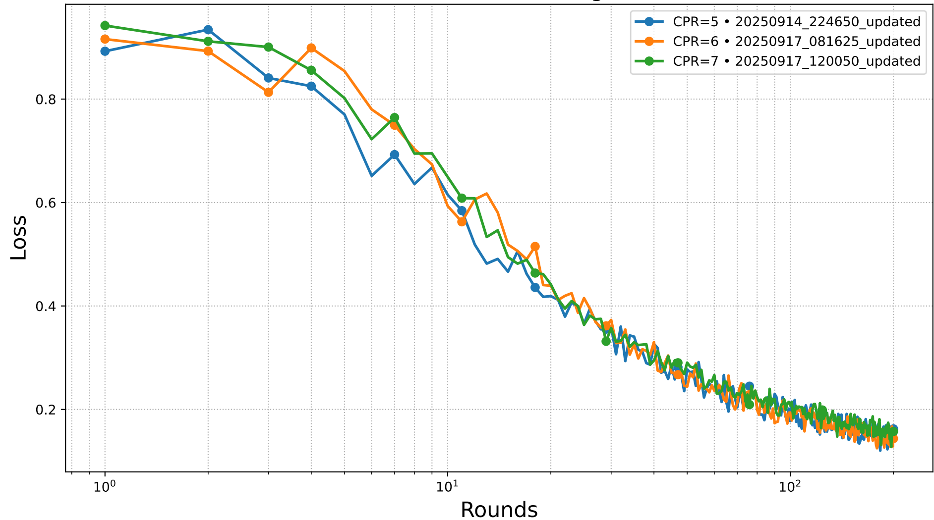
CIFAR-10 • RAFL • Server Loss (avg client train loss)
