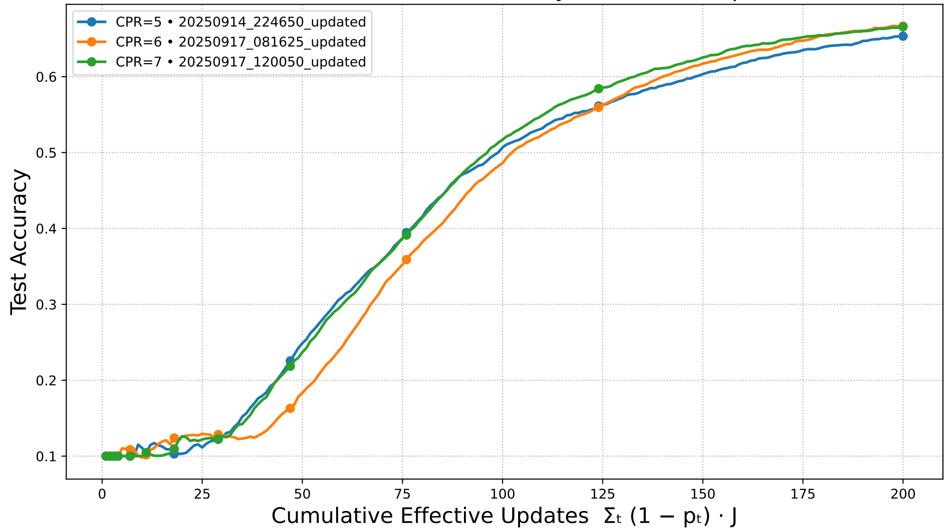
CIFAR-10 • RAFL • Test Accuracy vs Effective Updates
