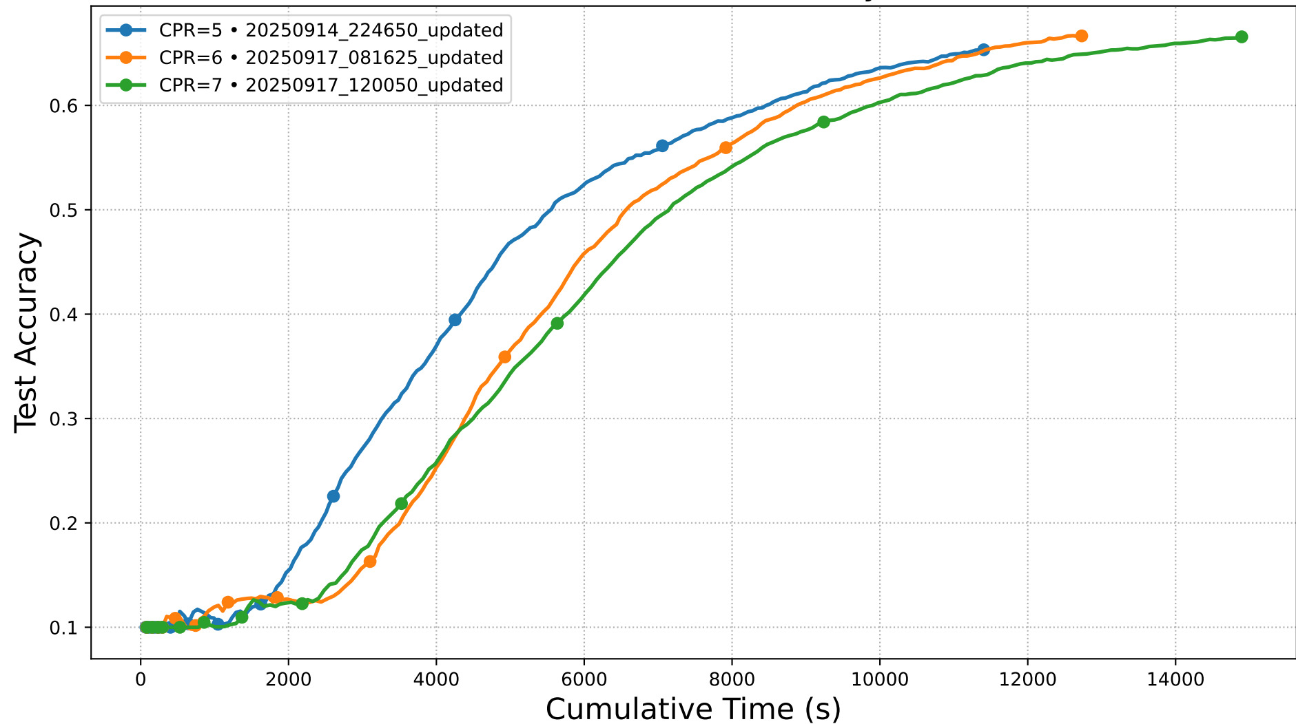
CIFAR-10 • RAFL • Test Accuracy vs Time
