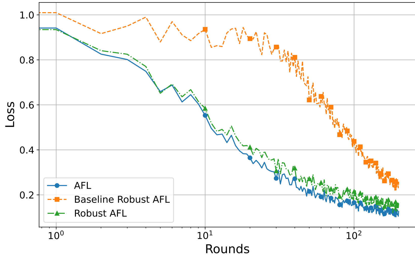
CIFAR Server Loss
