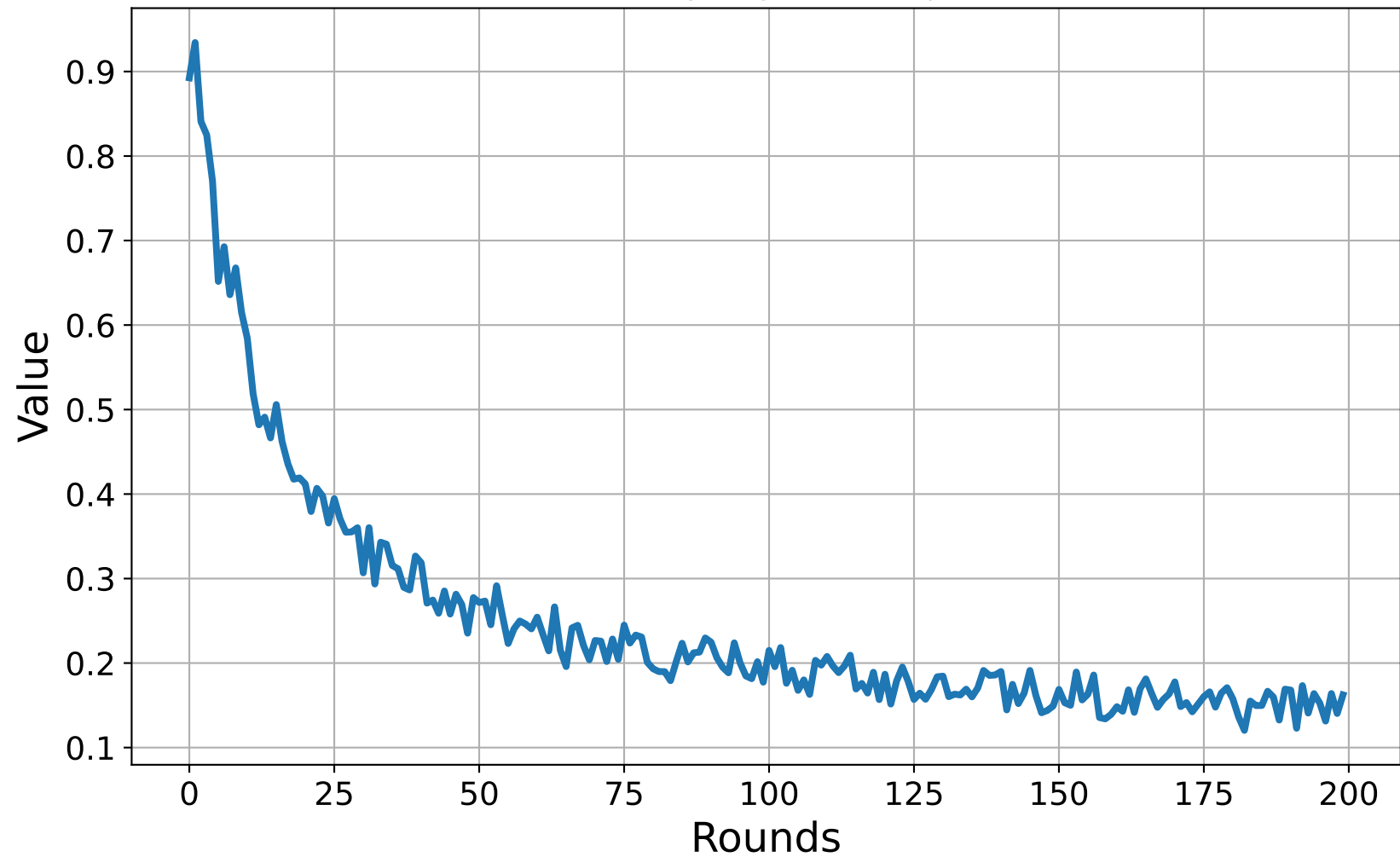
Server Loss Proxy (avg client loss per round)
