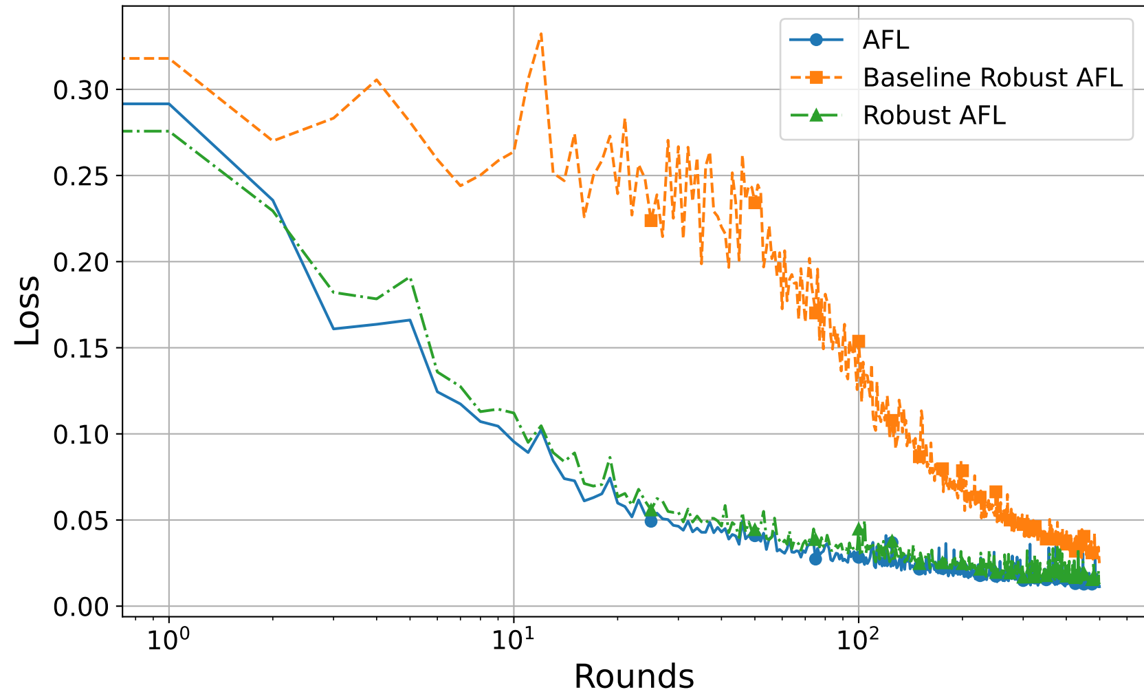
MNIST Server Loss
