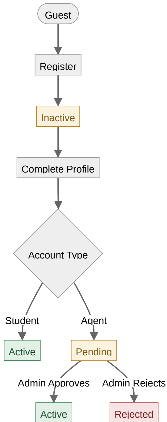
Figure 2. Account status lifecycle.
