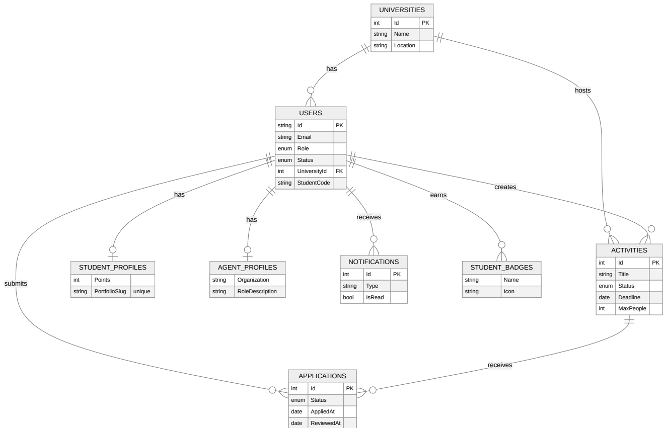
Figure 3. Conceptual data model (entity relationships).
