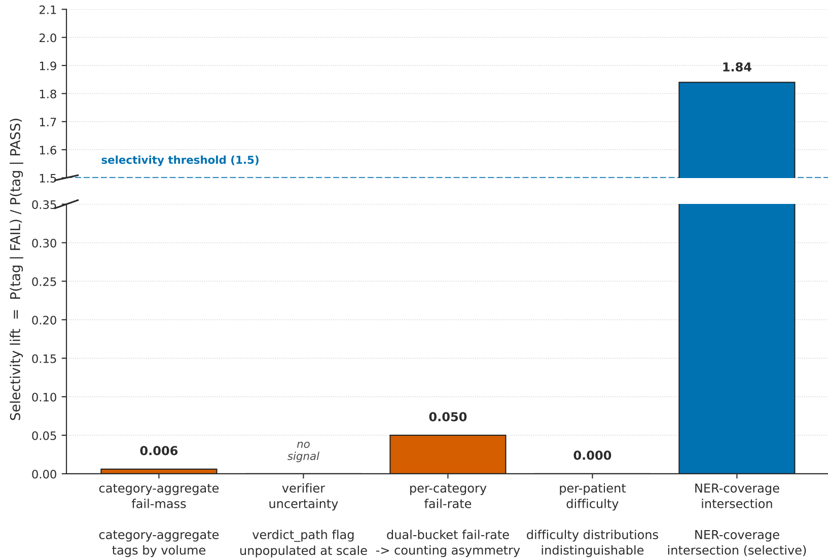
Five signal sources for the question-answering gate: one structurally aligned signal
