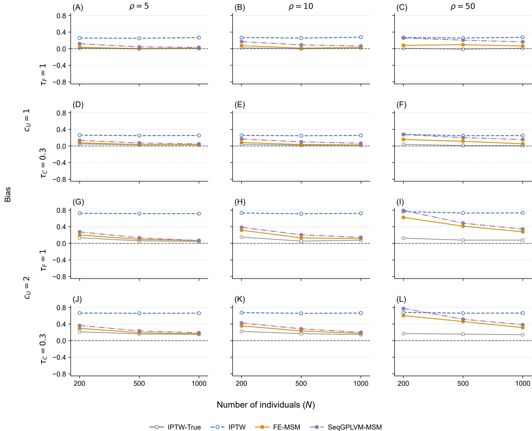
Simulation bias in the four-covariate case
