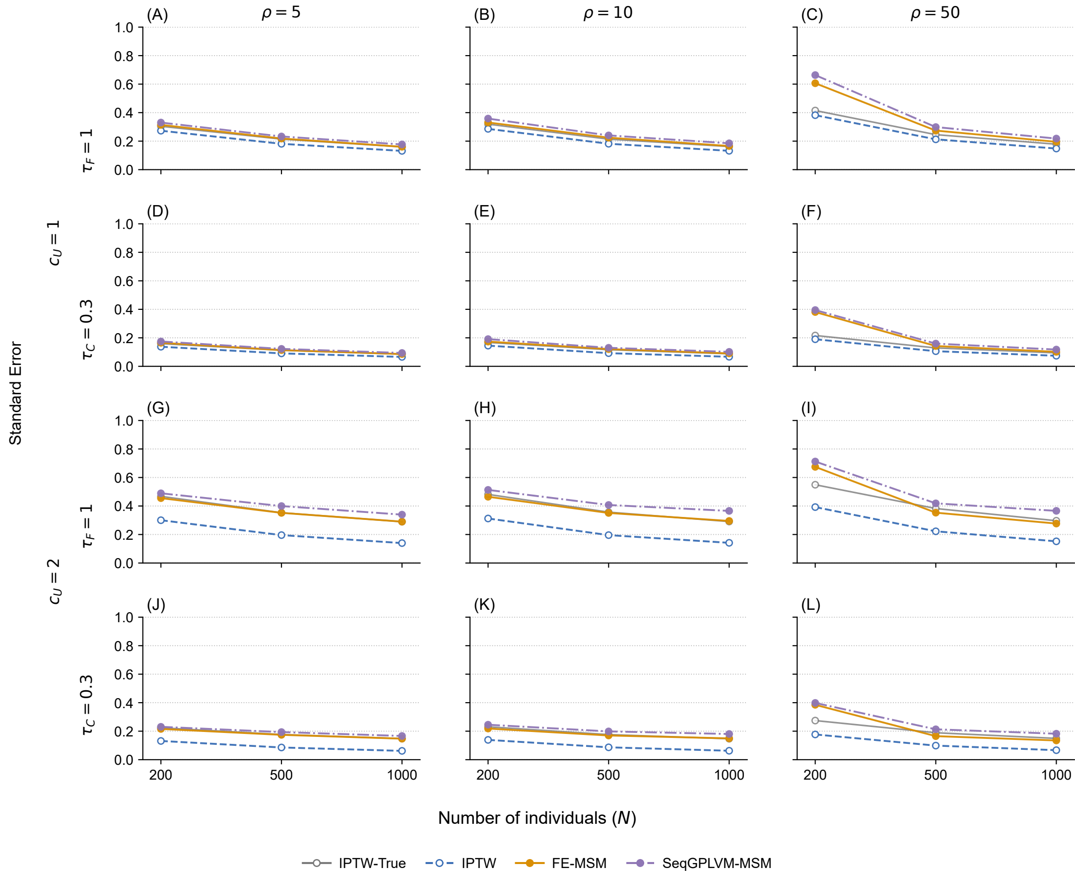
Average estimated standard errors in the four-covariate case
