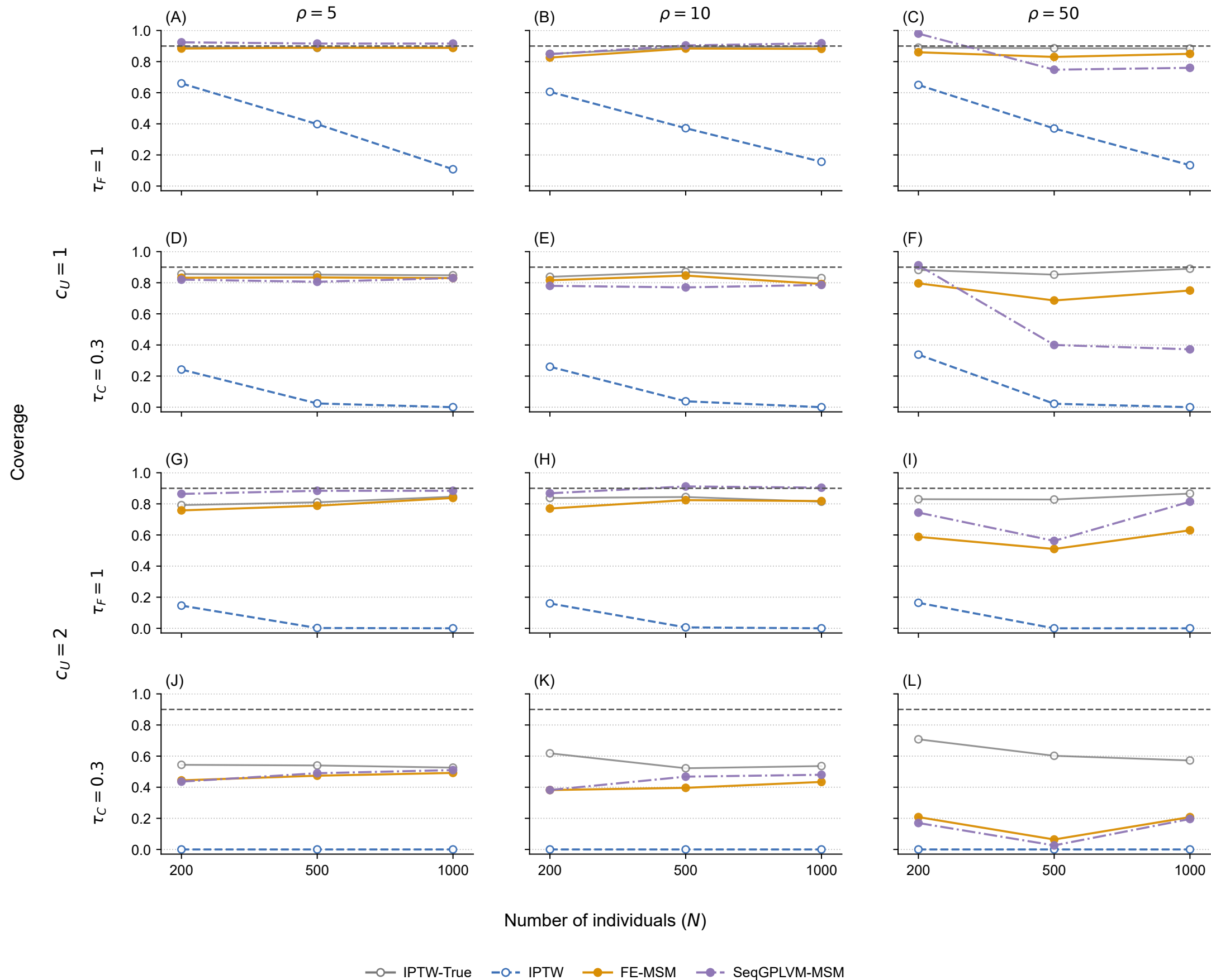
Coverage of 90% confidence intervals in the two-covariate case
