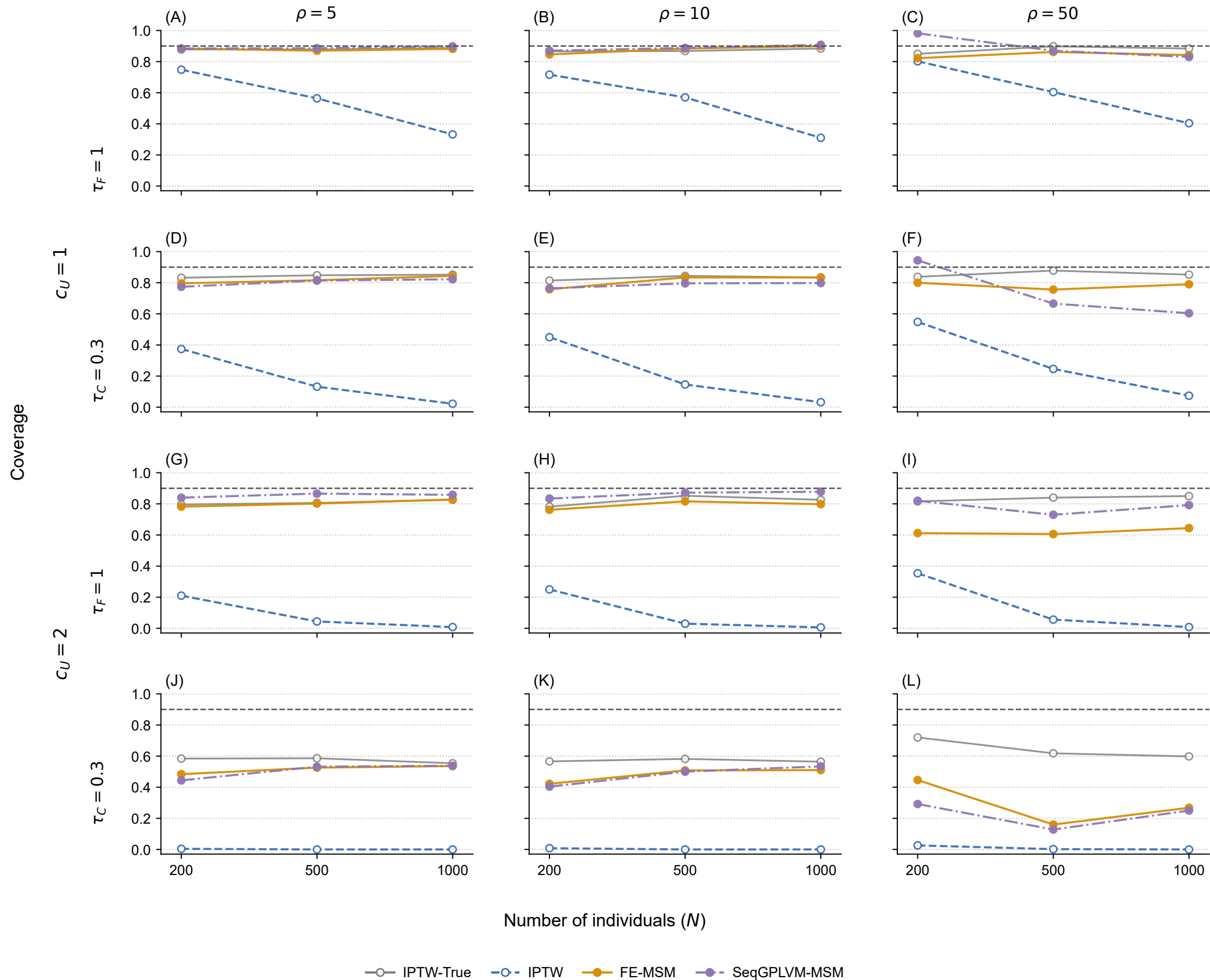
Coverage of 90% confidence intervals in the four-covariate case
