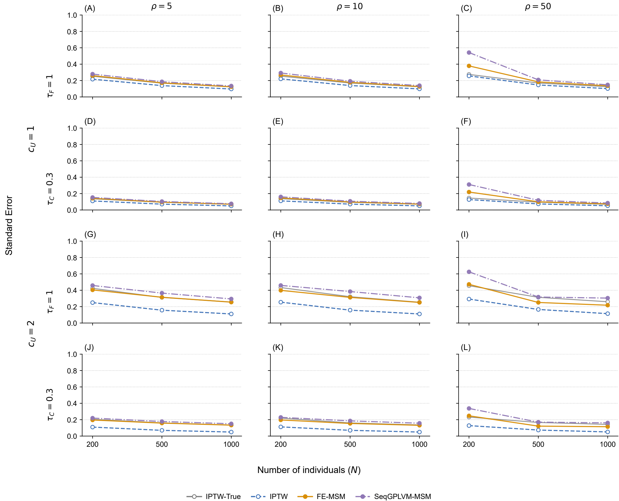
Average estimated standard errors in the two-covariate case
