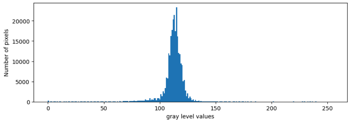
Contrast stretch
