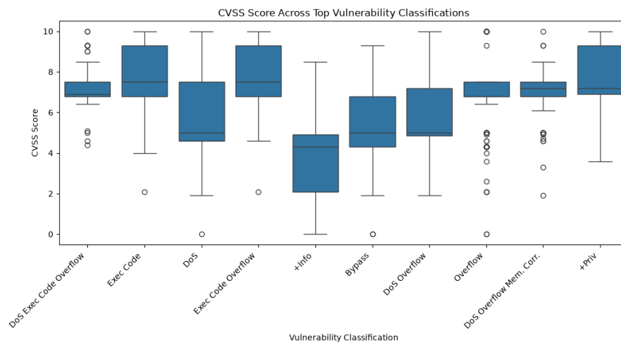
Figure 5. CVSS score distribution across the most frequent vulnerability classification categories.
