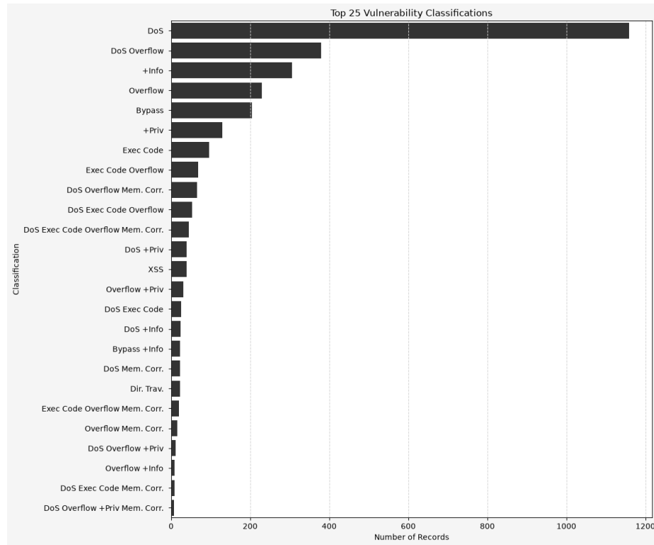
Figure 2. Top 25 vulnerability_classification categories by record count.
