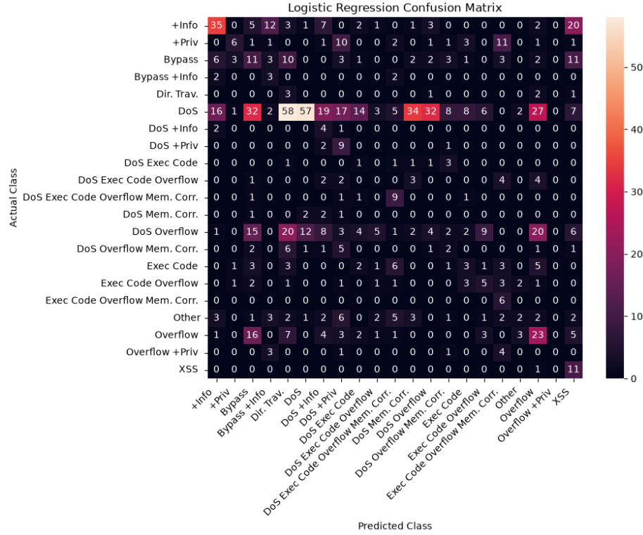
Figure 9. Confusion matrix for the multiclass vulnerability-classification model.
