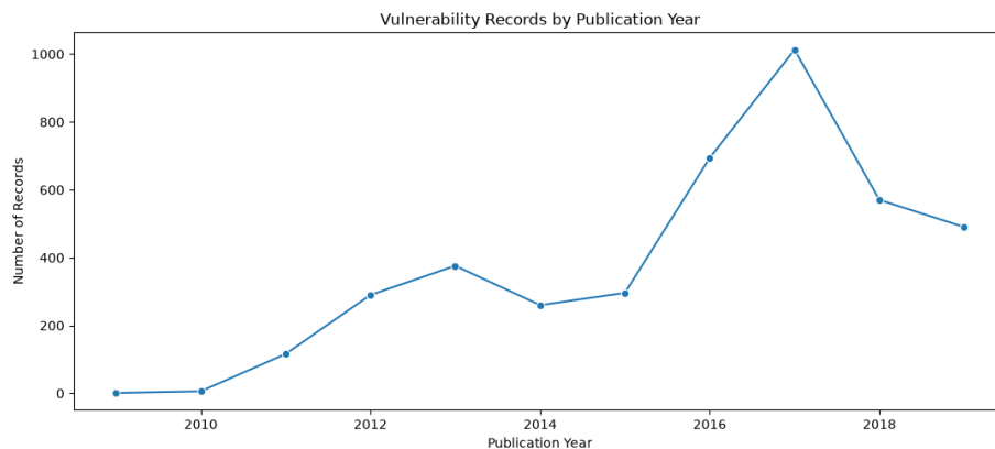
Figure 3. Number of vulnerability records by publication year (2009–2019).
