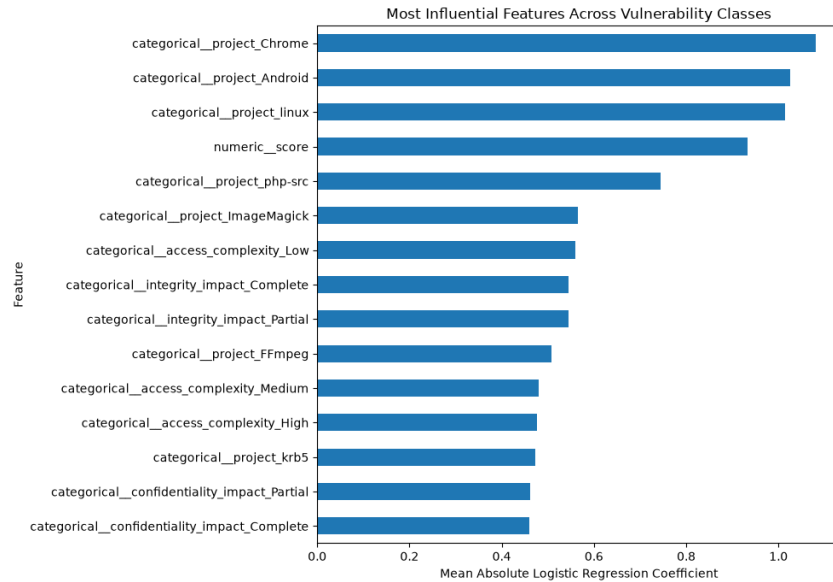
Figure 10. Mean absolute coefficient magnitude by feature (Logistic Regression).
