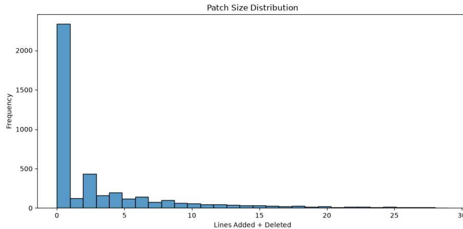
Figure 7. Distribution of lines changed per vulnerability-fixing commit (95th-percentile trimmed).
