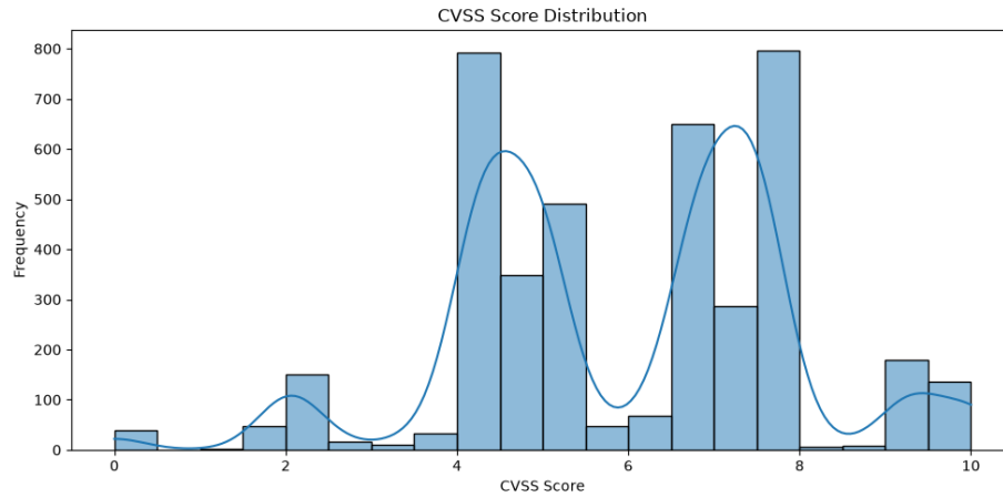
Figure 4. Distribution of CVSS severity scores across all records.
