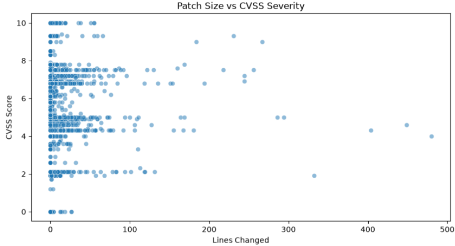
Figure 8. Relationship between lines changed and CVSS score.
