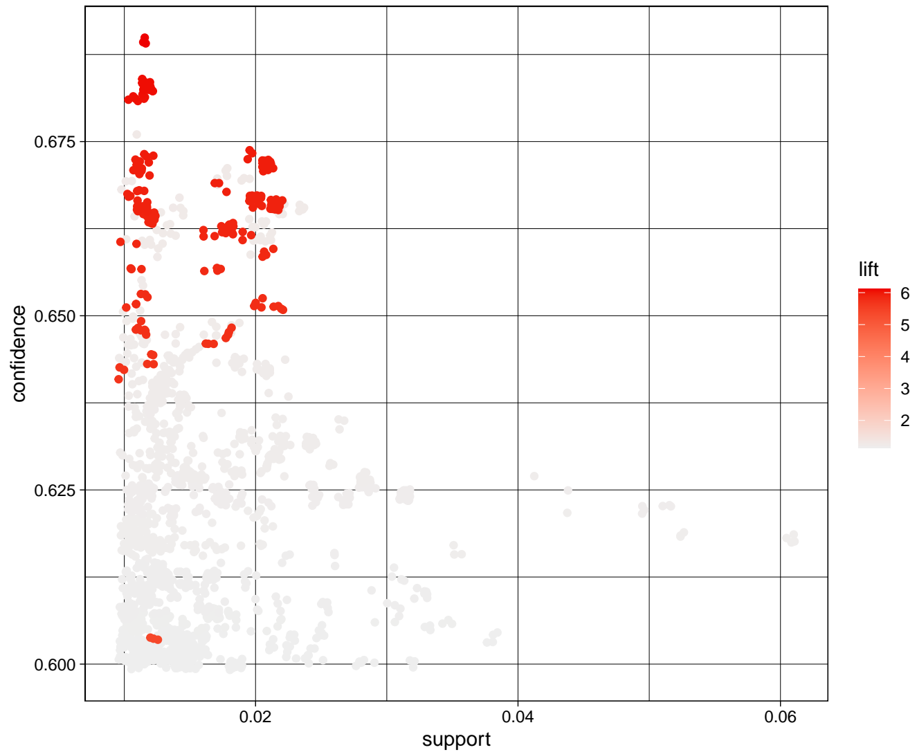
Scatter plot for 1587 rules
