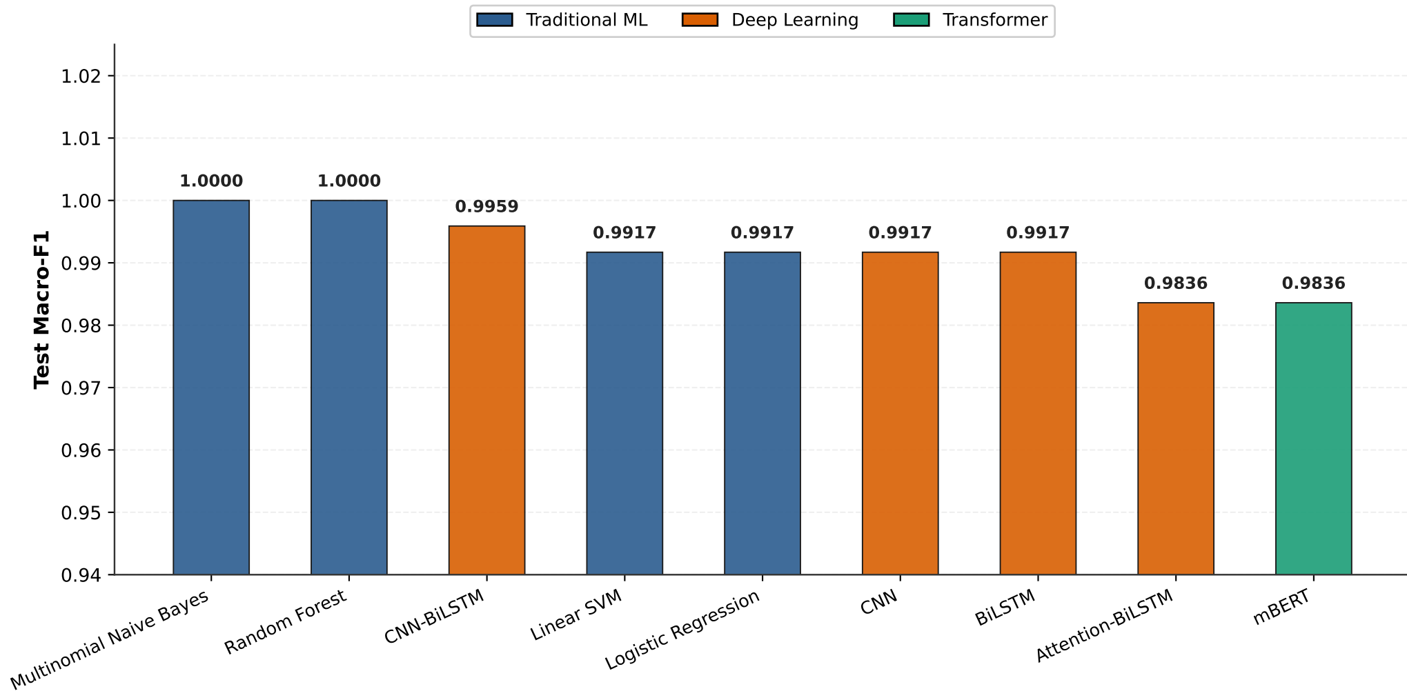
Test Macro-F1 Performance Across Model Families (N = 320)
