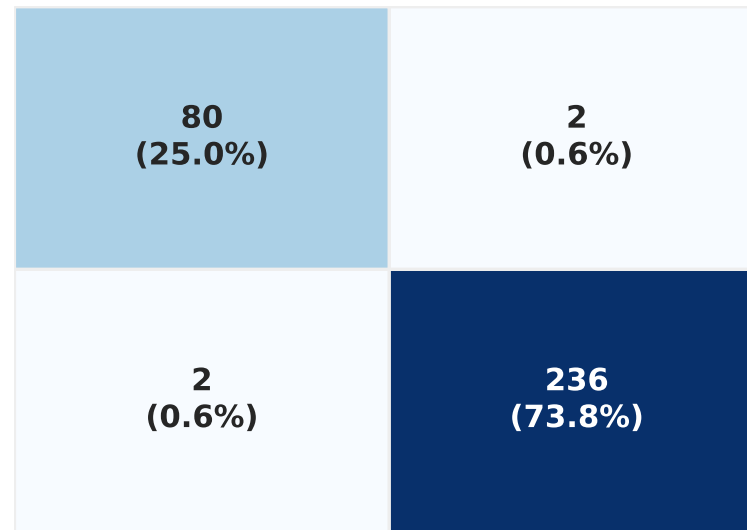
(e) Attention-BiLSTM [Deep Learning] Macro-F1: 0.9836
