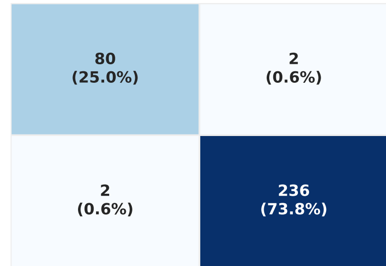
(f) mBERT [Transformer] Macro-F1: 0.9836
