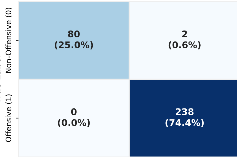
(a) Linear SVM [Traditional ML] Macro-F1: 0.9917
