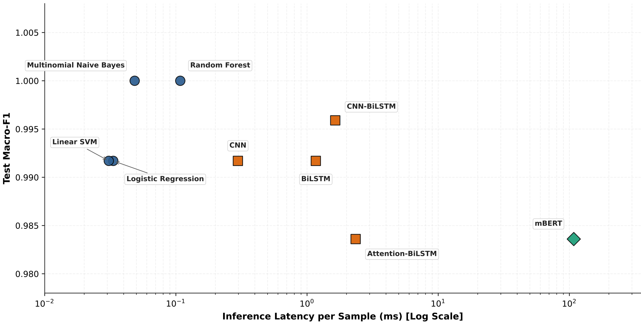
Performance vs. Inference Latency Trade-Off Across 9 Models
