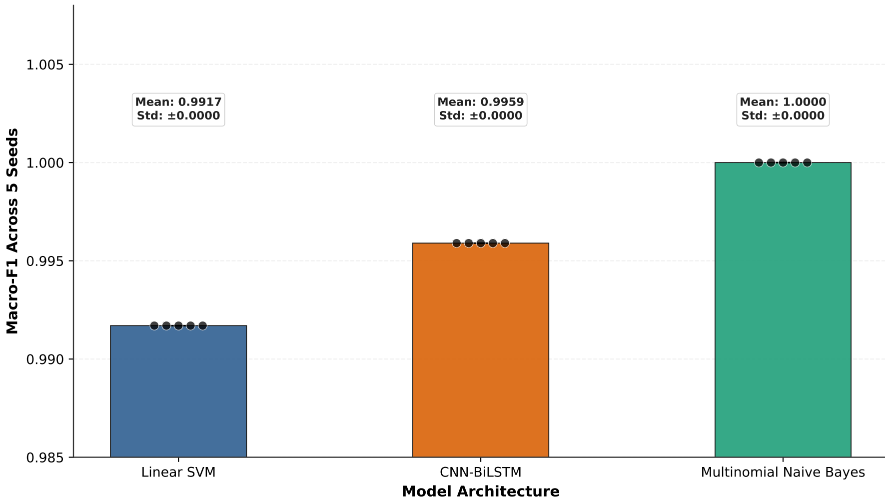
Repeatability Across 5 Random Seeds (42, 123, 456, 789, 2026)
