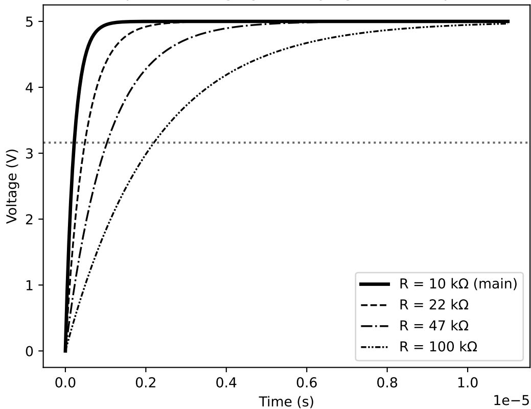
Capacitor charging for varying R ( C = 22 \text{ pF} )
