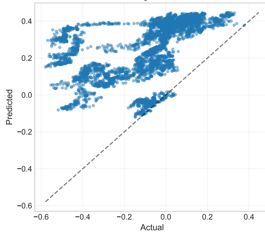
ae_lgbm
