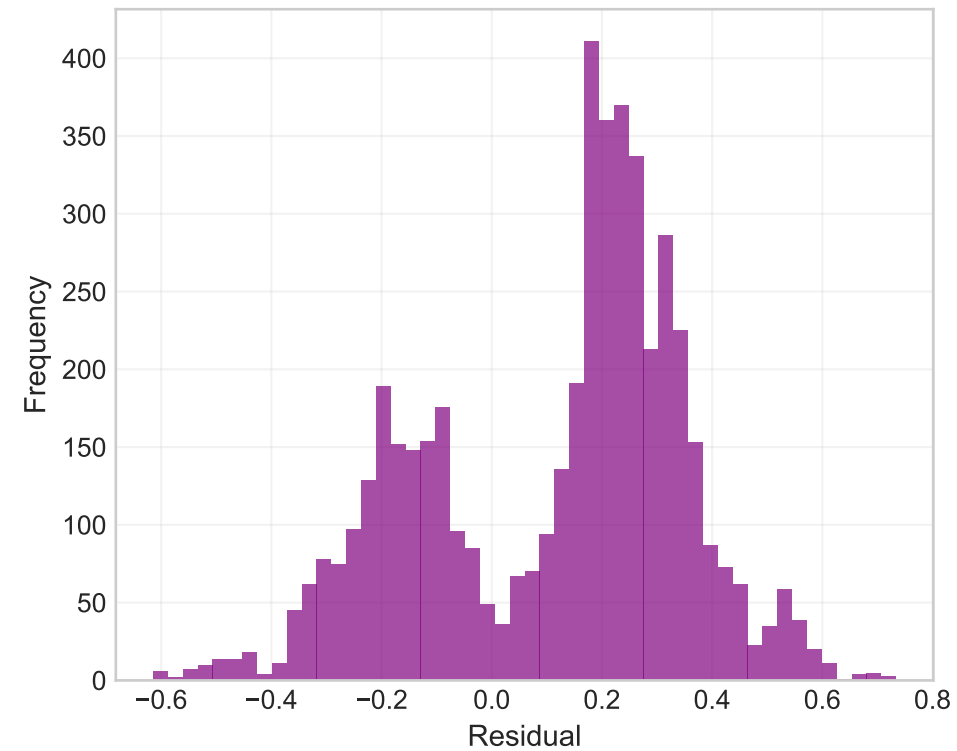
1M Residuals
