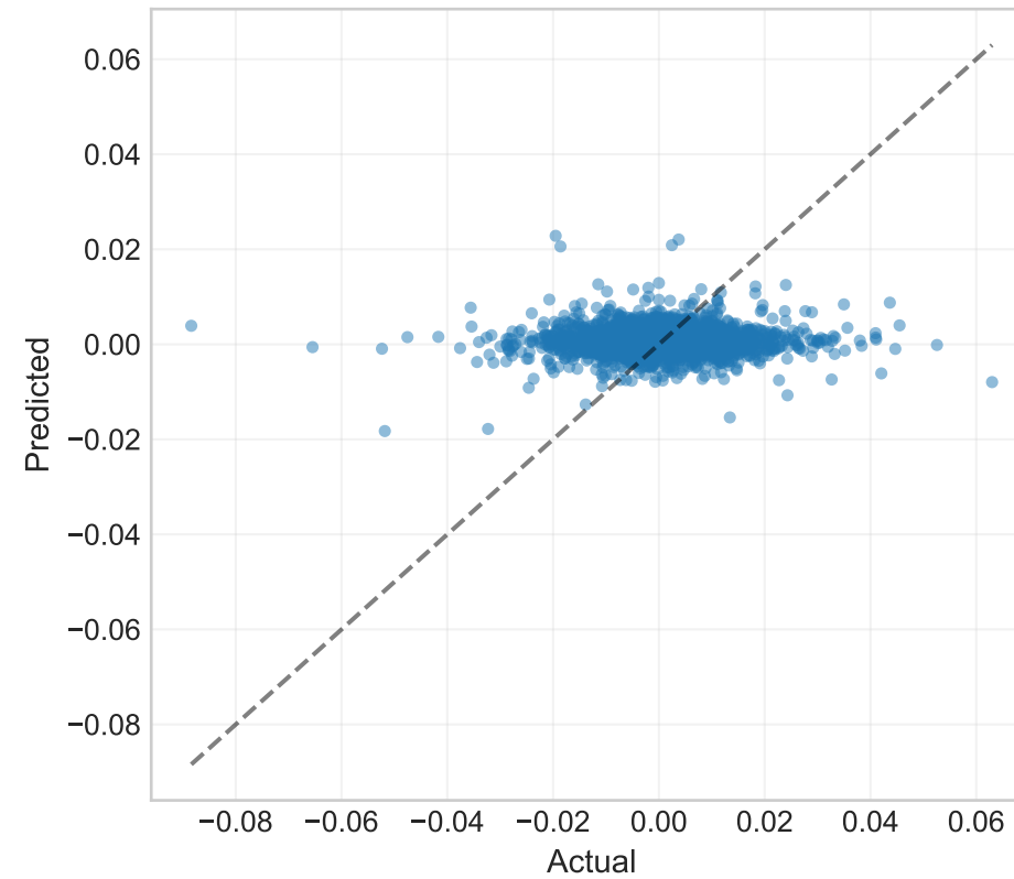
ae_lgbm
