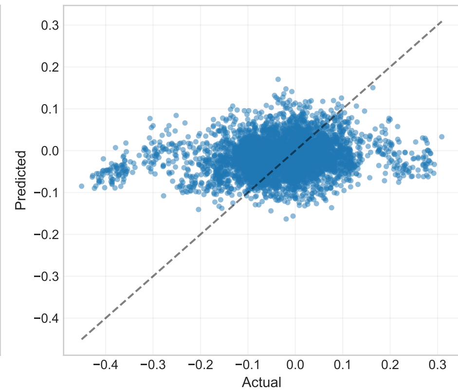
resnet
