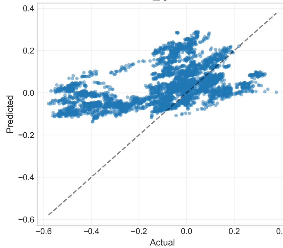
ae_lgbm
