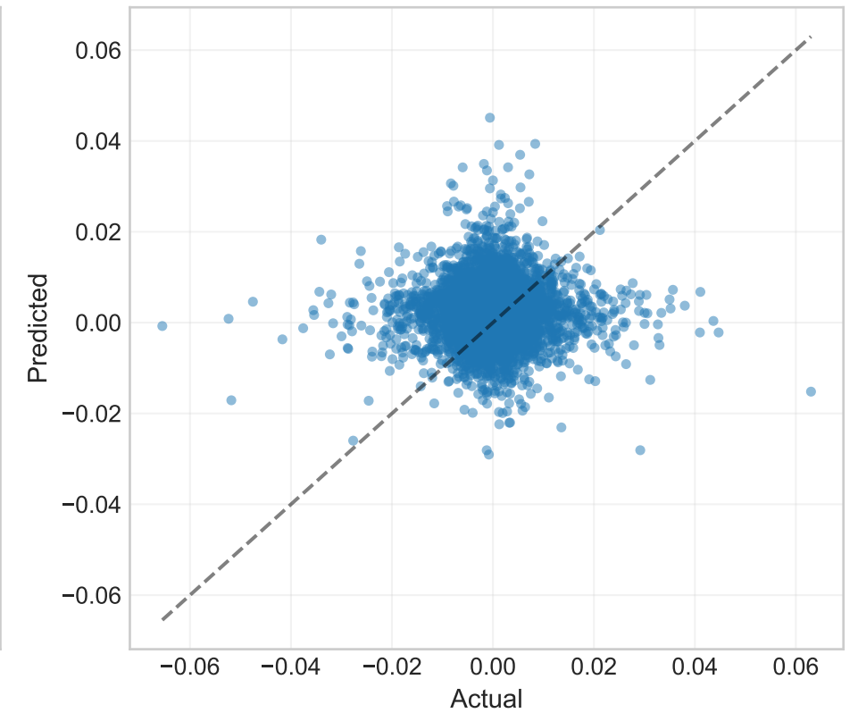
resnet
