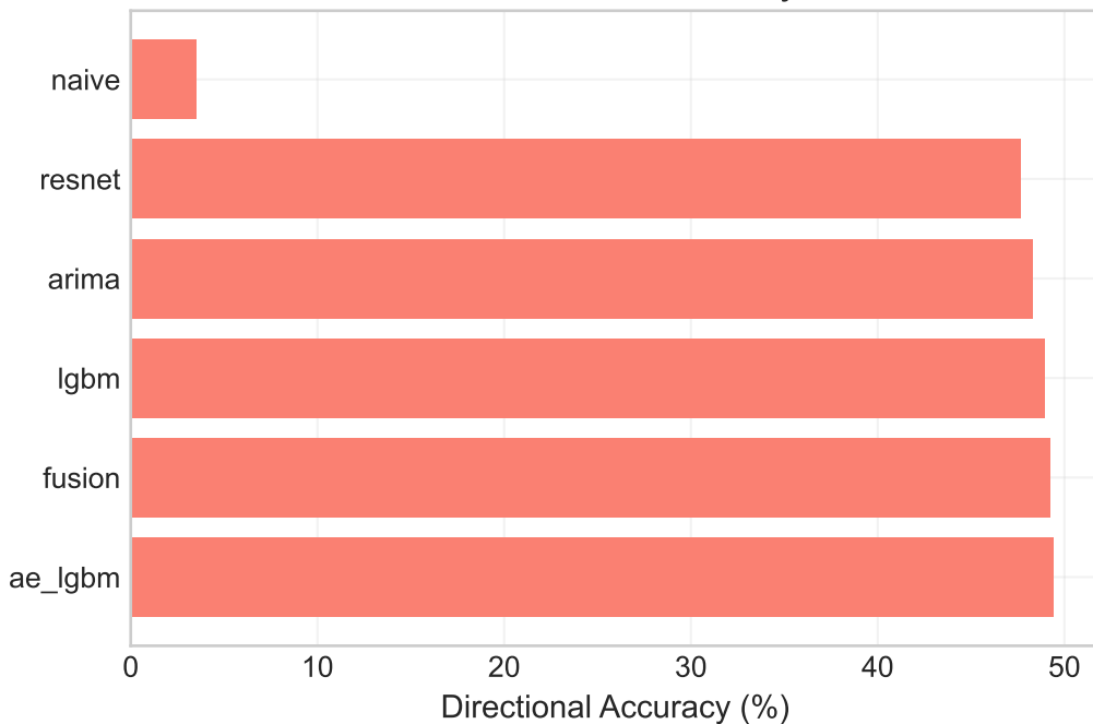
Directional Accuracy
