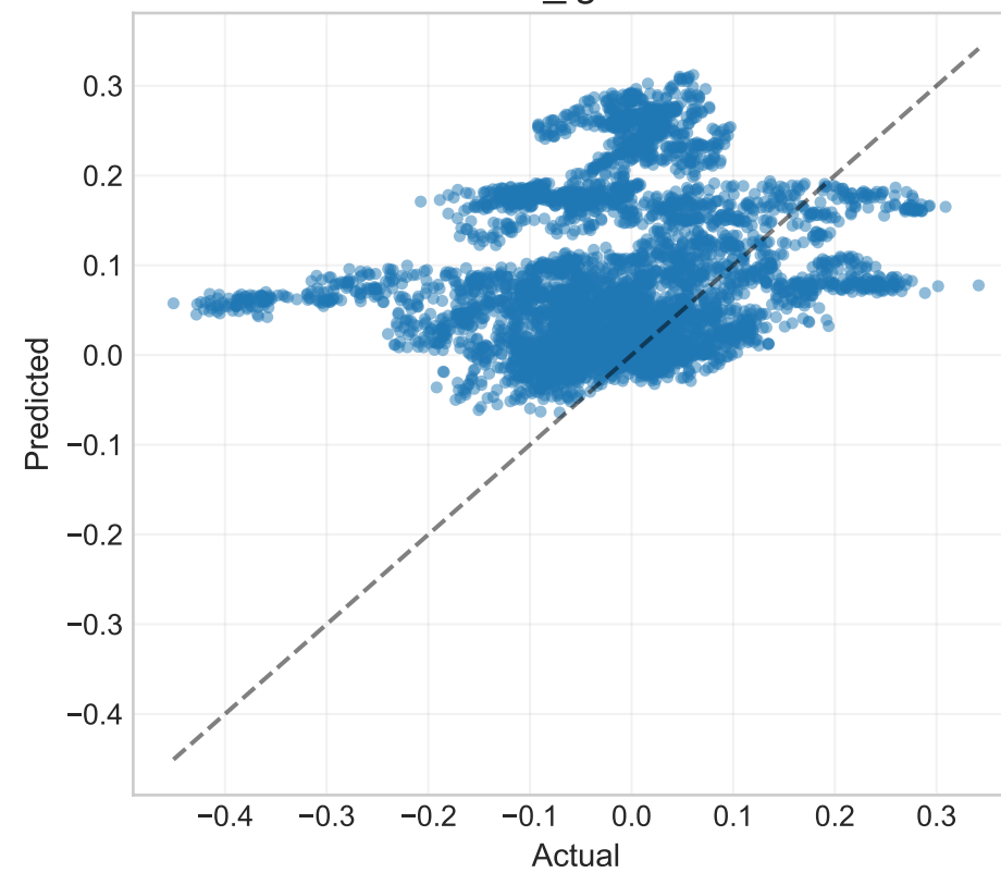
ae_lgbm
