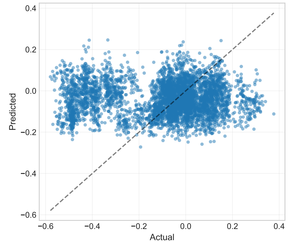
resnet
