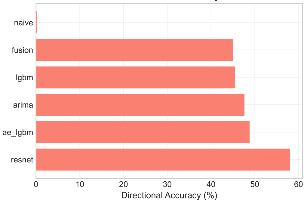
Directional Accuracy
