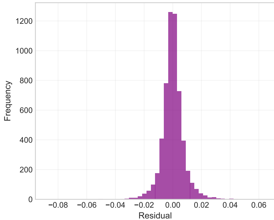
1H Residuals
