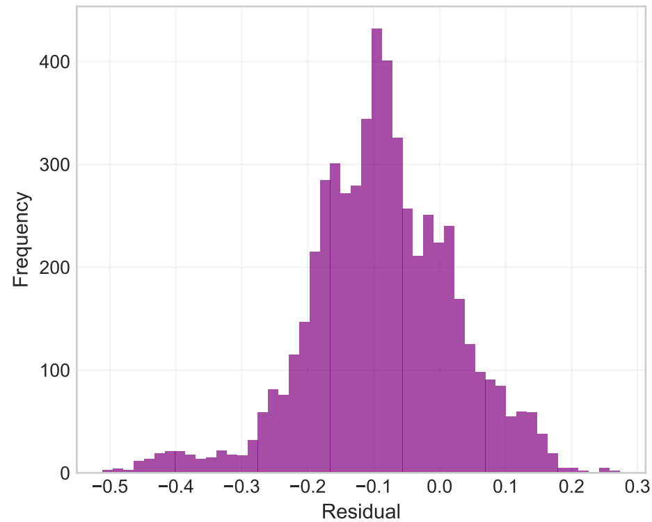
1W Residuals
