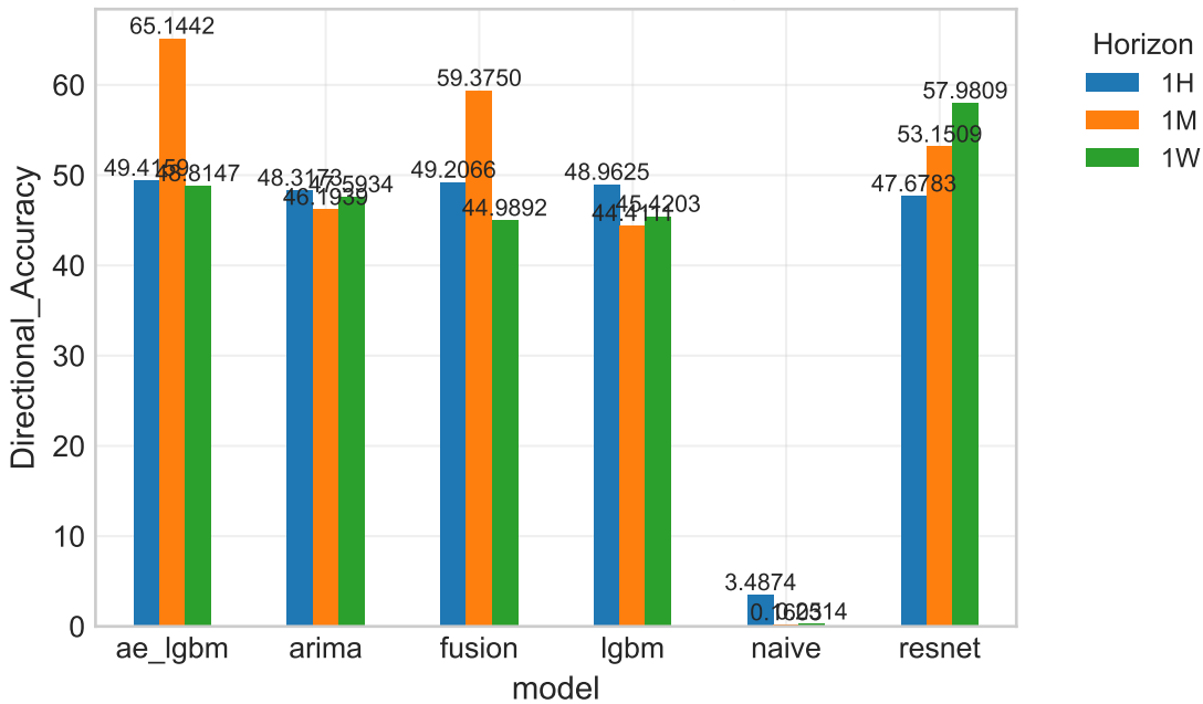
Directional_Accuracy
