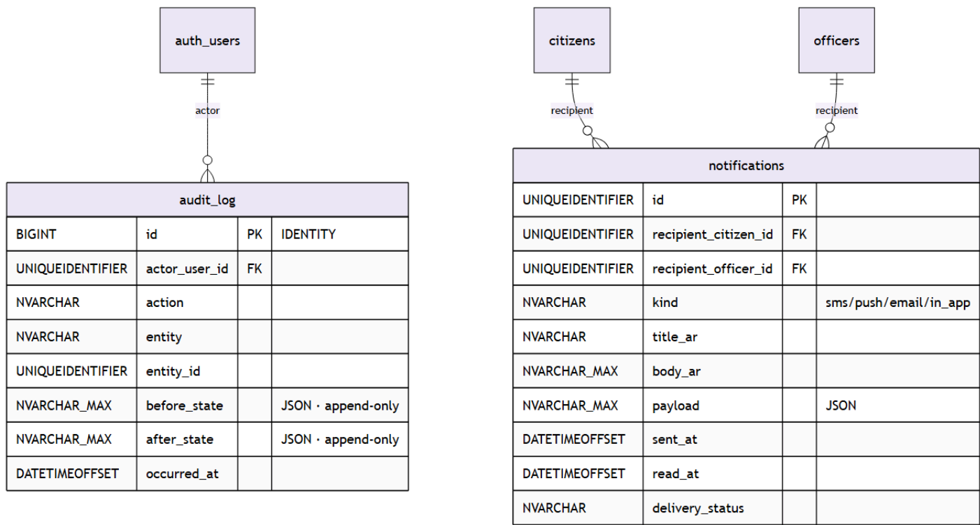
Sarh — Logical ERD · System cluster (notifications, audit log)
