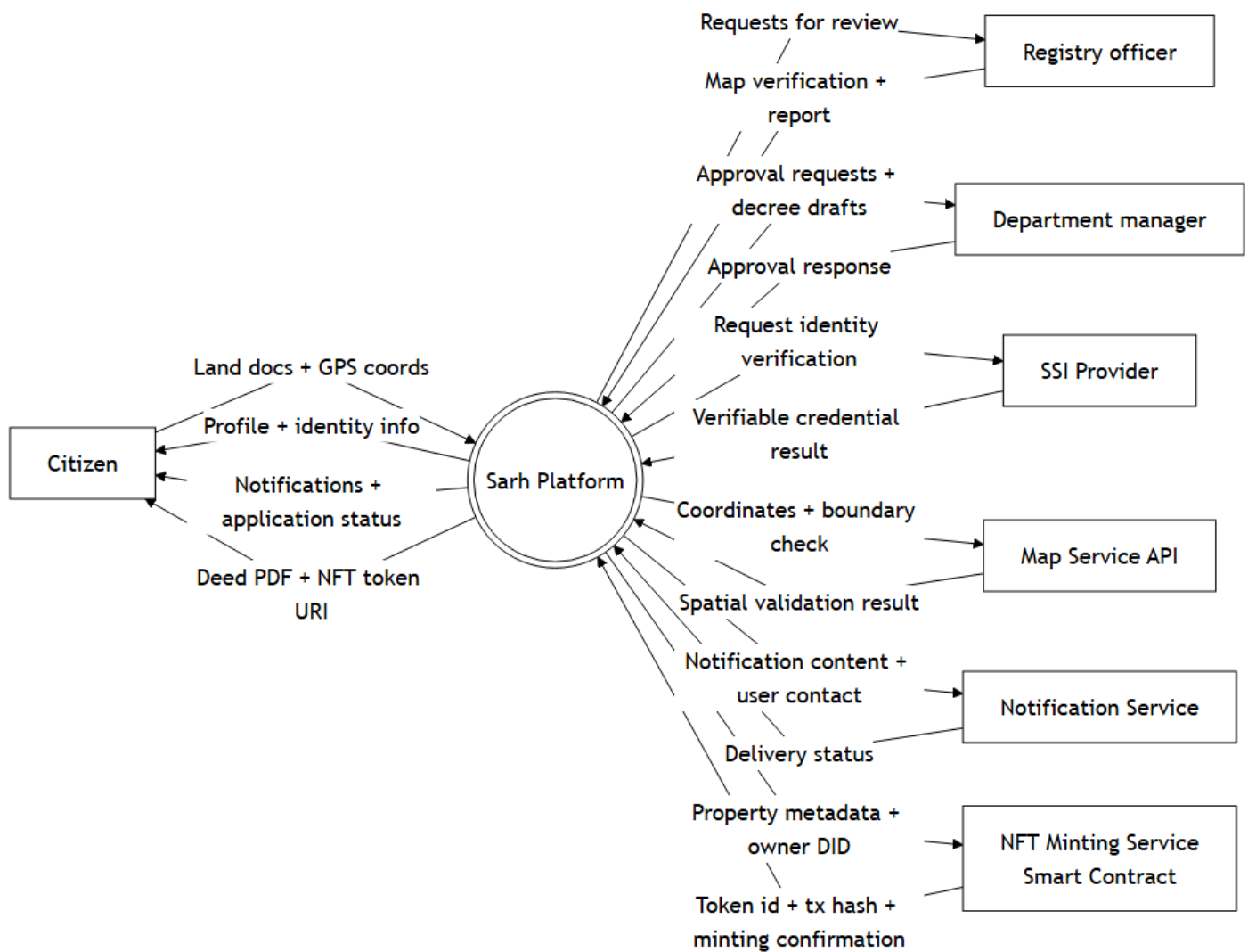
Sarh — Data-flow Context diagram (DFD Level 0 / Single process)
