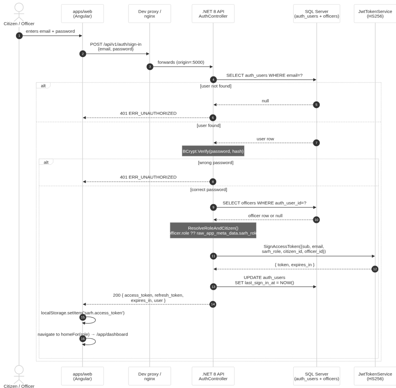
Sarh — Sign-in sequence (POST /api/v1/auth/sign-in)
