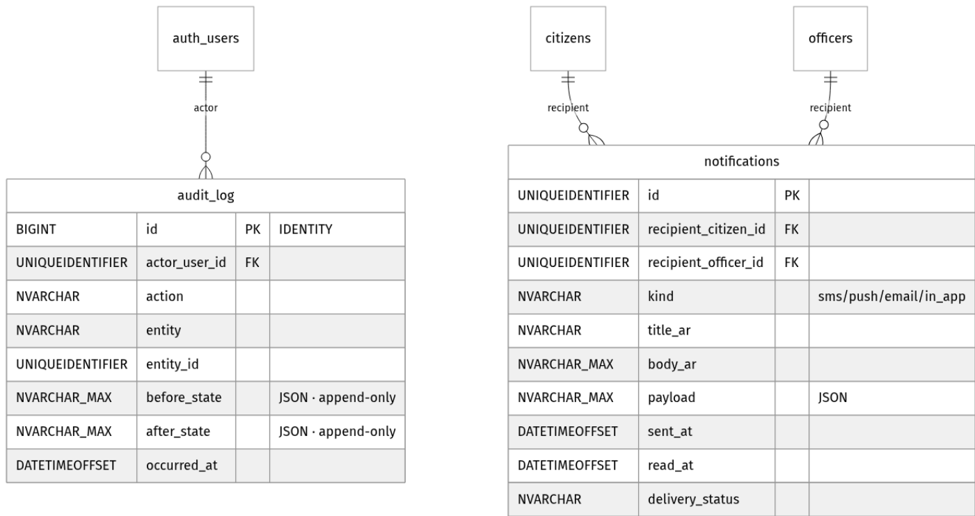
Sarh — Logical ERD · System cluster (notifications, audit log)
