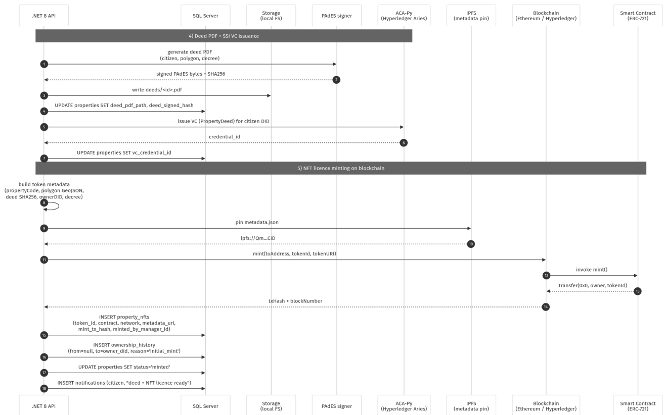
Sarh — Property approval (2/3) · Deed PDF + SSI VC + IPFS + NFT mint
