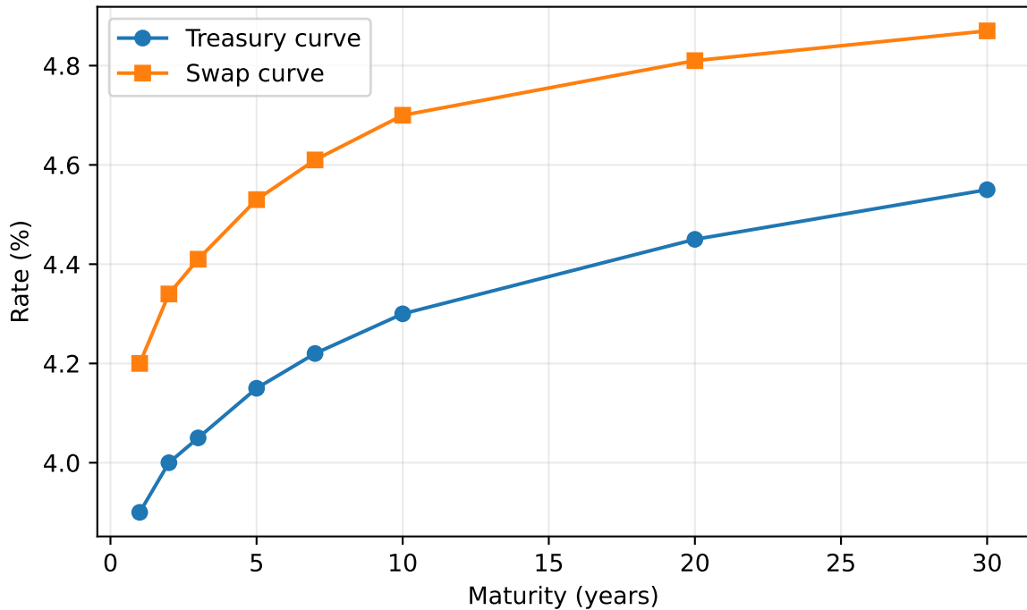
Swap Rate Yield Curve
