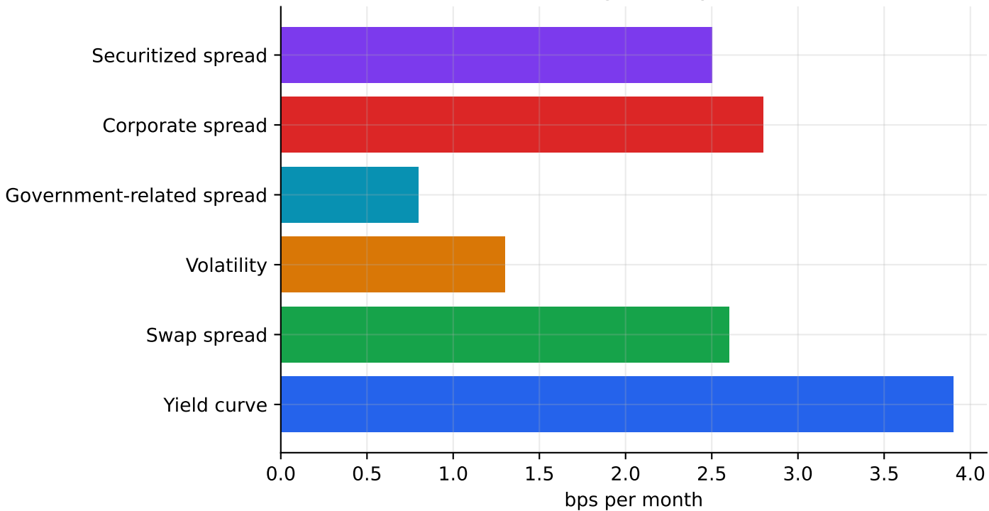
Isolated Tracking Error by Risk Factor
