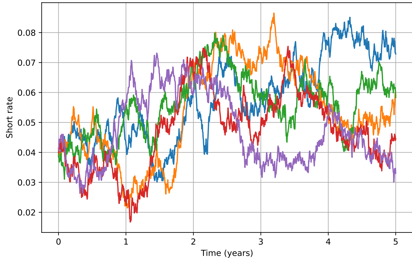
Ornstein-Uhlenbeck (Vasicek) process simulations
